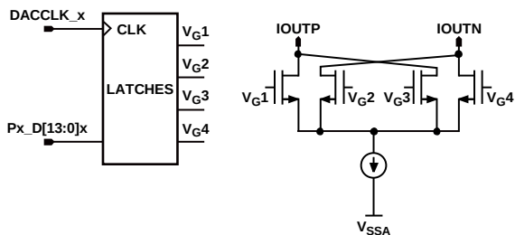
Figure 143. Quad-Switch Architecture
