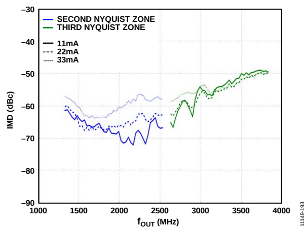
Figure 93. IMD vs. f_{OUT} over DAC I_{OUTFS}
