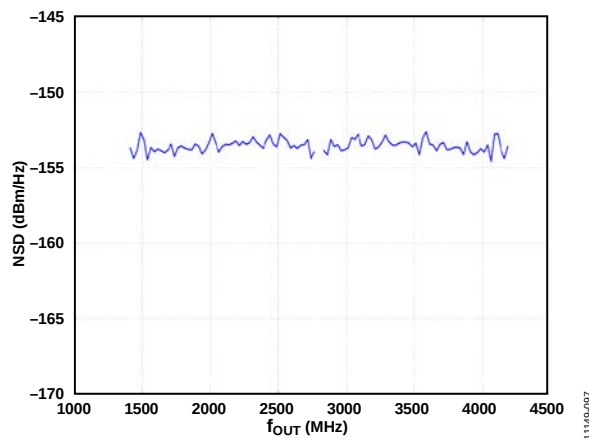
Figure 86. Single-Tone NSD vs. f_{OUT}
