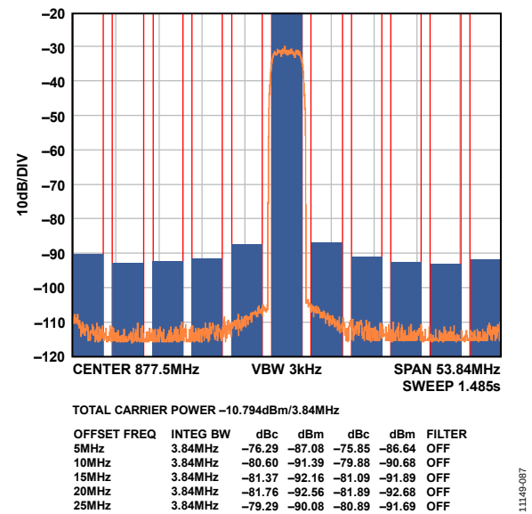
Figure 76. Single-Carrier W-CDMA at 877.5 MHz
