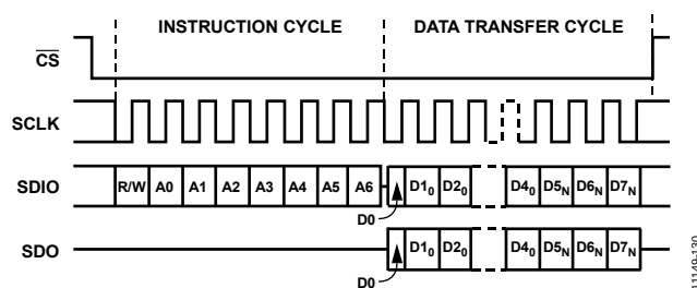
Figure 125. Serial Register Interface Timing, LSB-First Read
