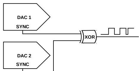
Figure 135. Example of Synchronization of Two DACs to \pm 1 DACCLK Accuracy
