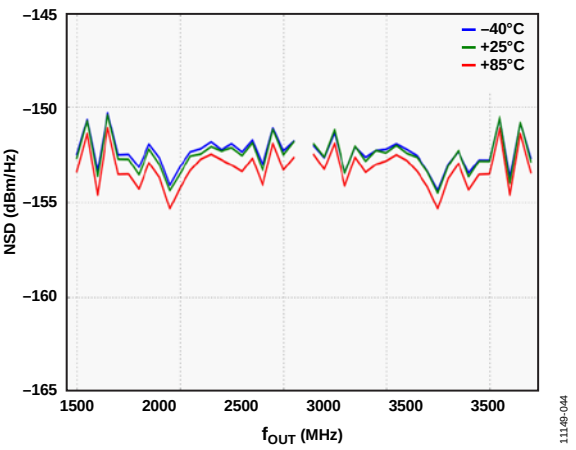
Figure 36. W-CDMA NSD vs. f_{OUT} over Temperature
