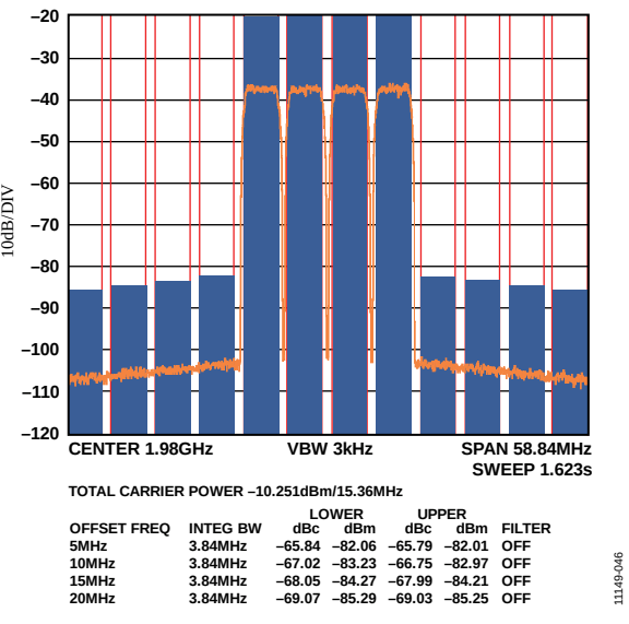
Figure 37. Four-Carrier W-CDMA at 1980 MHz
