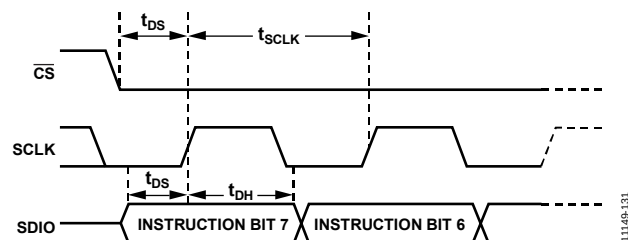
Figure 126. Timing Diagram for an SPI Register Write
