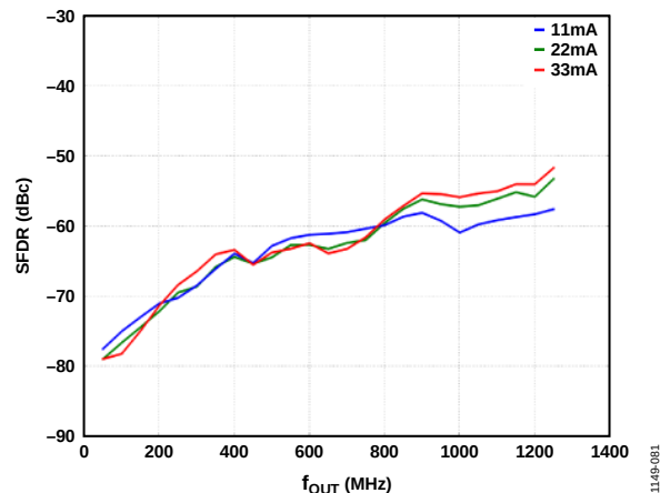
Figure 72. SFDR vs. f_{OUT} over DAC I_{OUTFS}
