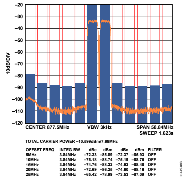
Figure 79. Two-Carrier W-CDMA at 875 MHz
