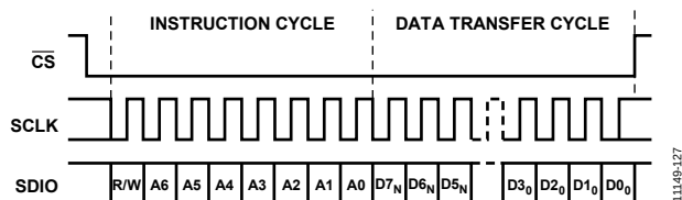
Figure 122. Serial Register Interface Timing, MSB-First Write
