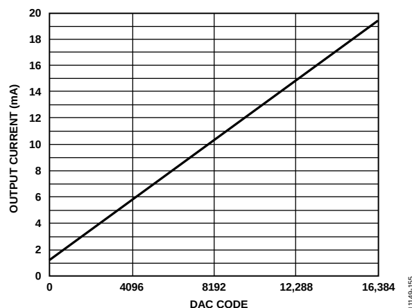
Figure 151. Gain Curve for FSC_x[9:0] = 512, DAC Offset = 1.228 mA
