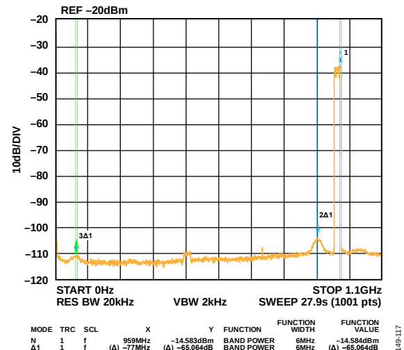
Figure 106. Four Carrier at 950 MHz Output
