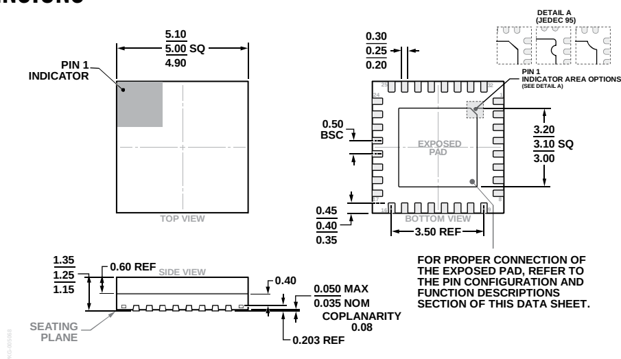
Figure 63. 32-Lead Lead Frame Chip Scale Package, Premolded Cavity [LFCSP_CAV] 5 mm × 5 mm Body and 1.25 mm Package Height (CG-32-2)
