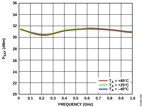
Figure 26. P_{SAT} vs. Low Frequency, 10 MHz to 1 GHz for Various Temperatures, Self Biased Mode, V_{DD} = 12\text{ V} , V_{GG1} = GND
