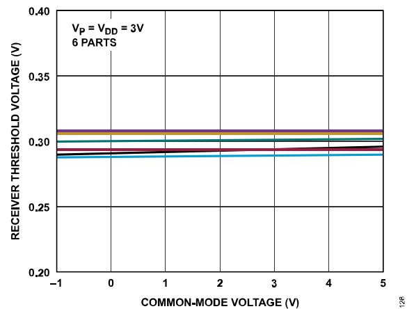
Figure 29. Receiver Threshold Voltage vs. Common-Mode Voltage at 3 V Supply
