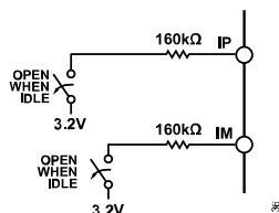
Figure 37. Receiver Common-Mode Bias
