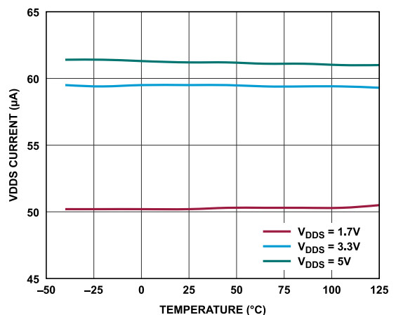
Figure 18. VDDS Current vs. Temperature, Ready State
