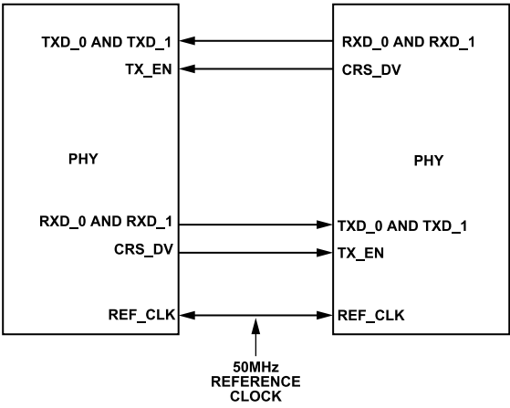
Figure 33. Back to Back with RMII Interface
