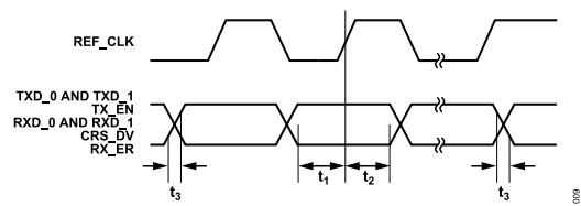
Figure 9. RMII Timing
