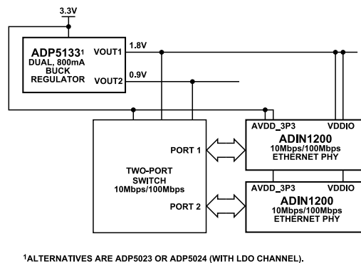
Figure 40. Recommended Power Solution for 3.3 V with RGMII Operating at VDDIO = 1.8 V
