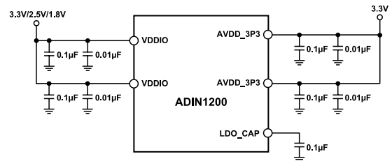
Figure 42. Supply Decoupling Overview
