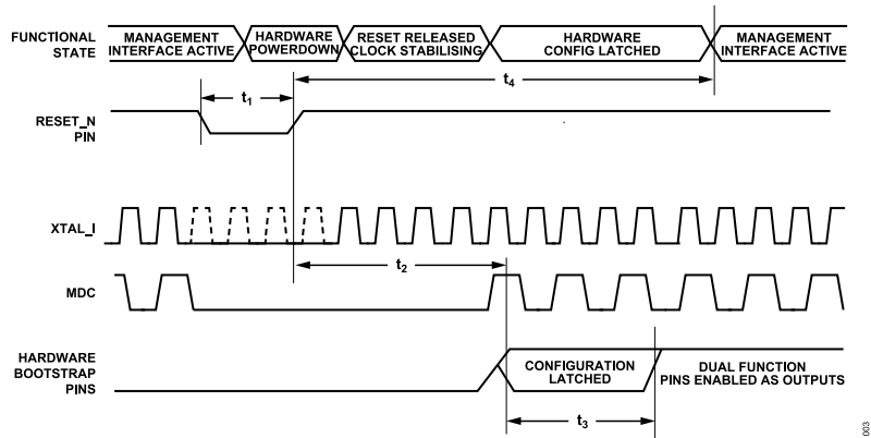
Figure 3. Hardware Reset Timing
