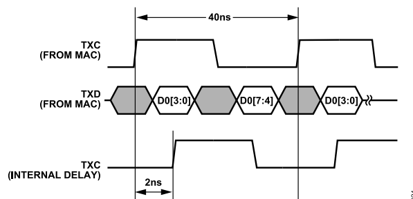
Figure 22. DLL Waveform
