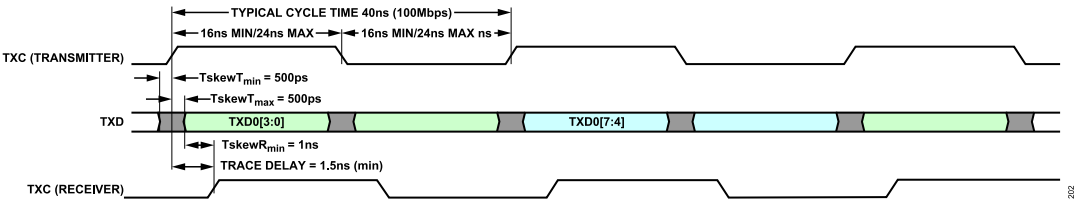
Figure 34. RGMII Timing Example for 100 Mbps Data Rate (Using PCB Trace Delay)
