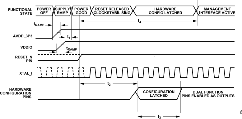
Figure 2. Power-Up Timing
