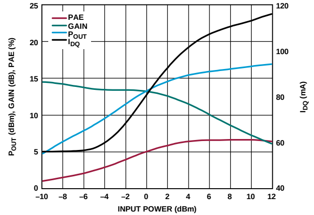
Figure 31. P_{OUT} , Gain, PAE, and I_{DQ} vs. Input Power, 26 GHz, V_{DD} = 5\text{ V}
