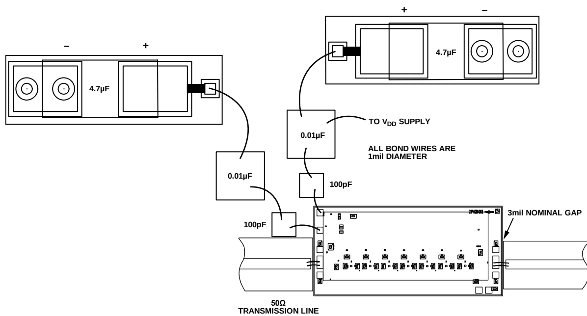
Figure 42. Assembly Diagram
