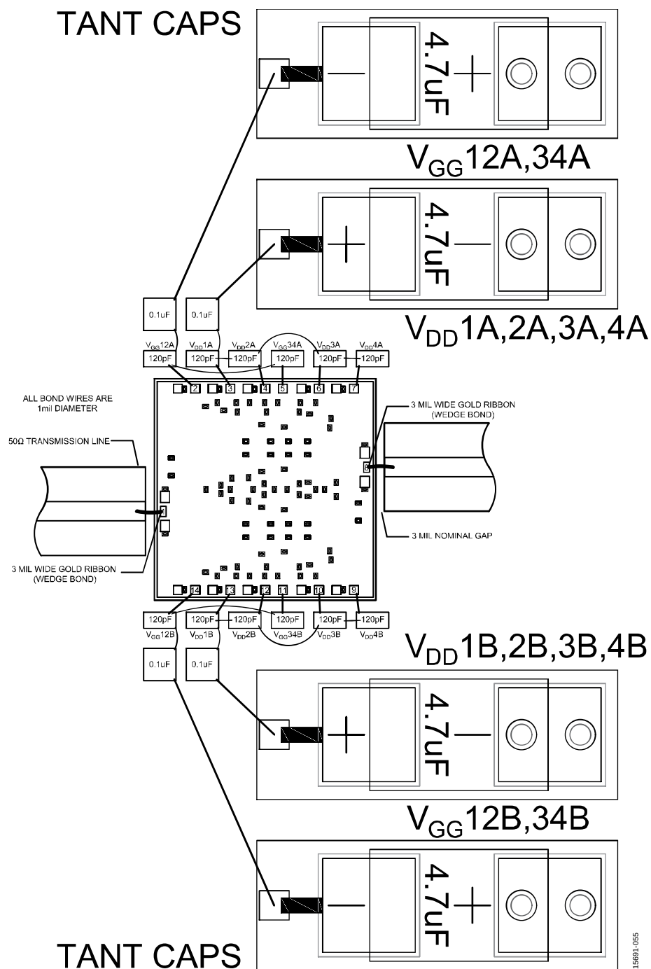
Figure 42. Assembly Diagram
