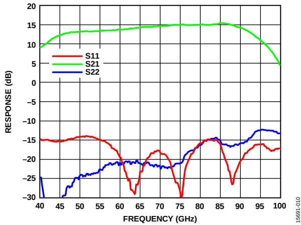
Figure 10. Broadband Gain and Return Loss vs. Frequency
