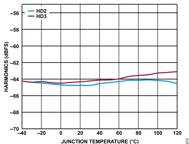
Figure 41. Harmonics vs. Junction Temperature, f_{IN} = 1.8 GHz, A_{IN} = -1 dBFS
