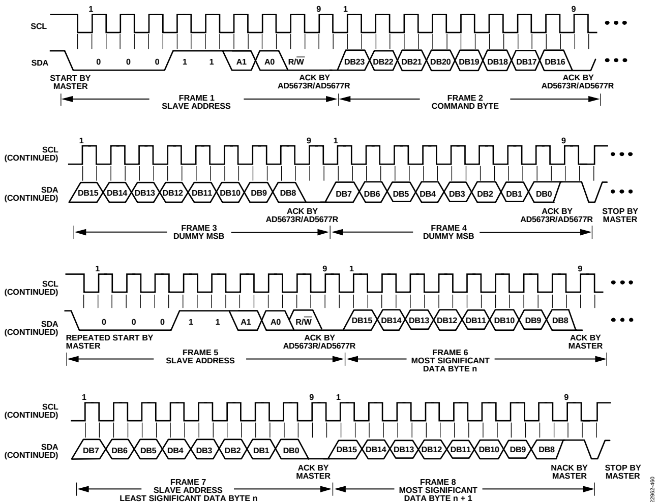
Figure 60. I²C Read Operation
