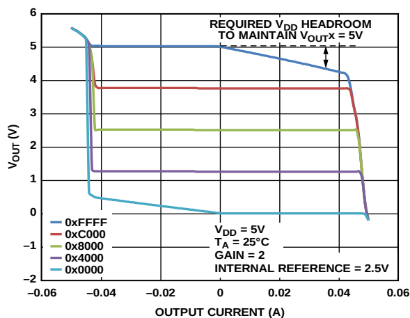
Figure 34. Source and Sink Capability at V_{DD} = 5V
