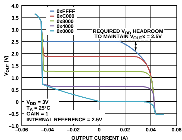
Figure 33. Source and Sink Capability at V_{DD} = 3V
