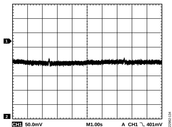
Figure 46. 0.1 Hz to 10 Hz Output Noise
