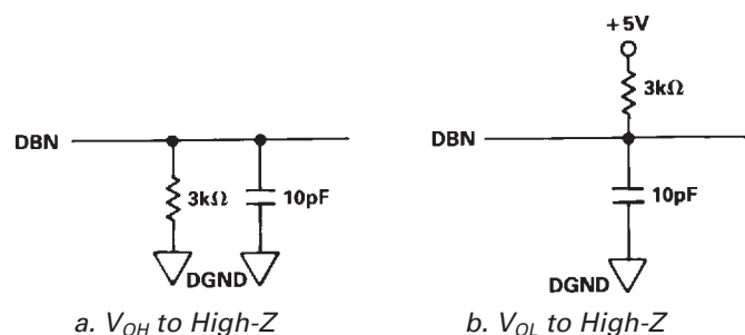
Figure 2. Load Circuits for Output Float Delay
