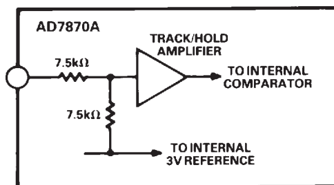
Figure 4. Analog Input
