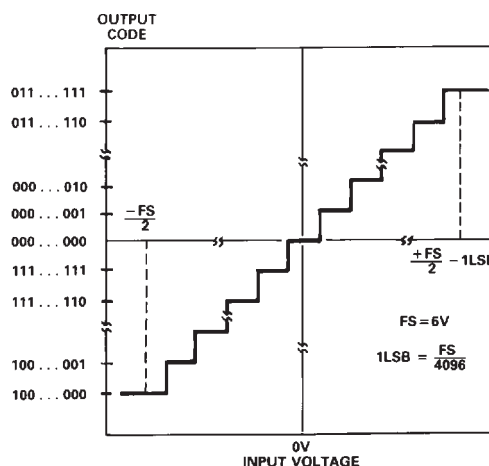
Figure 5. Bipolar Input/Output Transfer Function
