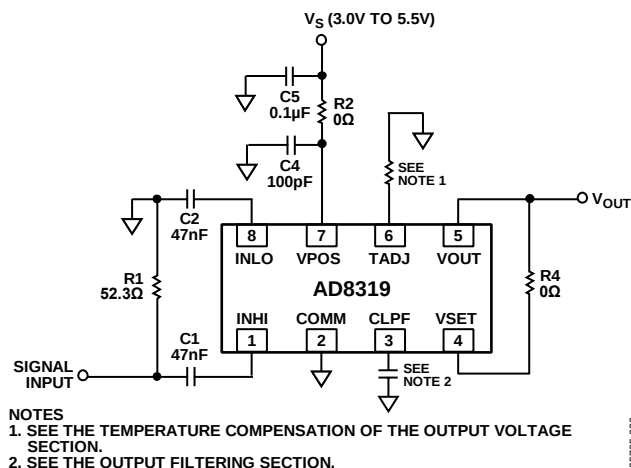
Figure 22. Basic Connections
