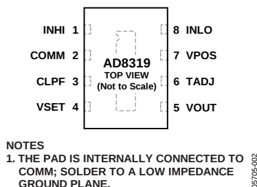
Figure 2. Pin Configuration
