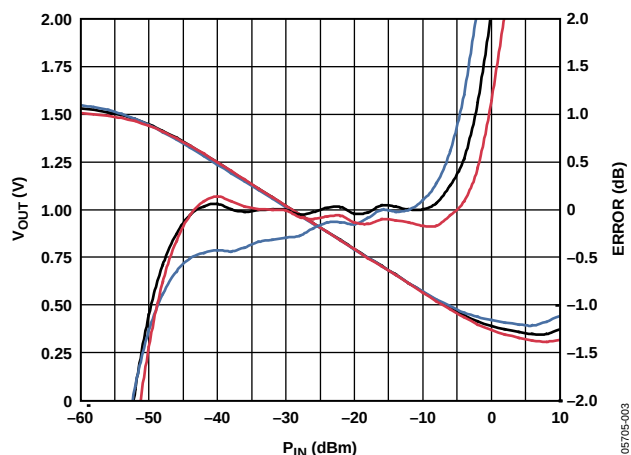
Figure 3. V_{OUT} and Log Conformance Error vs. Input Amplitude at 900 MHz, R_{TADJ} = 18\text{ k}\Omega
