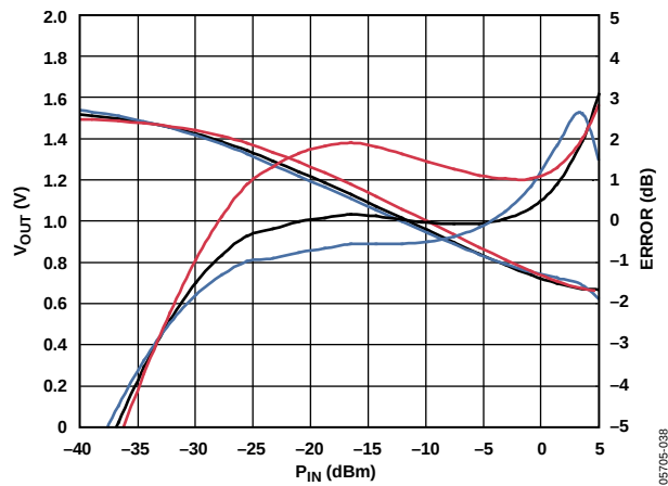
Figure 35. V_{OUT} and Log Conformance Error vs. Input Amplitude at 10 GHz, Multiple Devices, R_{TADJ} = Open, C_{LFP} = 1000 pF
