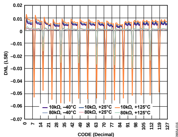
Figure 15. DNL vs. Code (AD5111)
