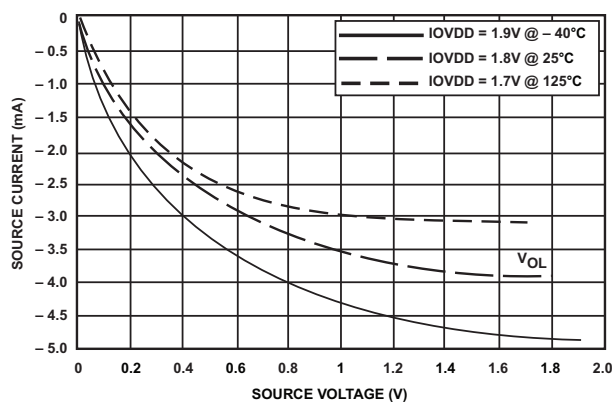
Figure 30. I 2 C Drivers (1.8 V IOVDD)
