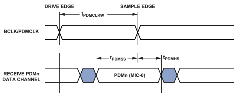
Figure 19. PDM Timing
