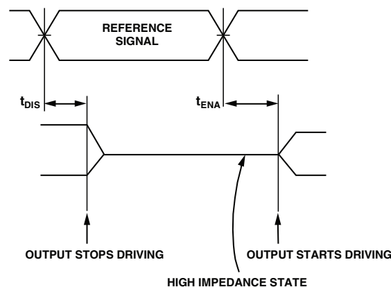
Figure 35. Output Enable/Disable
