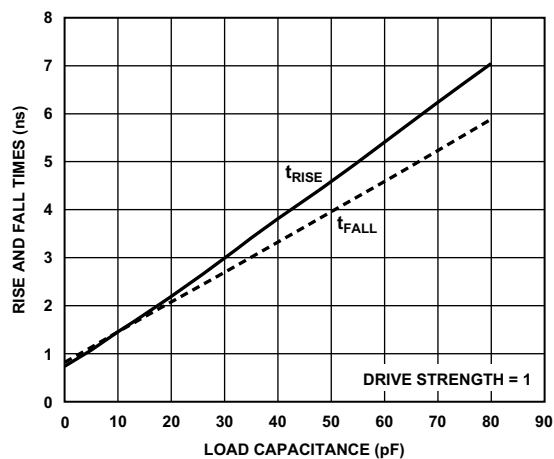
Figure 40. Digital I/O Driver Typical Rise and Fall Times (10% to 90%) vs. Load Capacitance ( V_{IODD} = 3.3\text{ V} , T_J = 25^\circ\text{C} )
