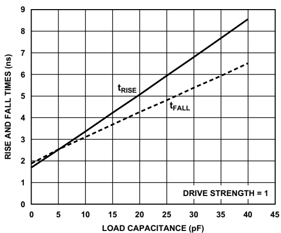
Figure 38. Digital I/O Driver Typical Rise and Fall Times (10% to 90%) vs. Load Capacitance ( V_{IODD} = 1.8\text{ V} , T_J = 25^\circ\text{C} )
