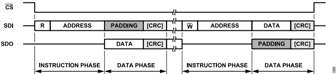
Figure 90. Single Instruction Mode SPI Frame
