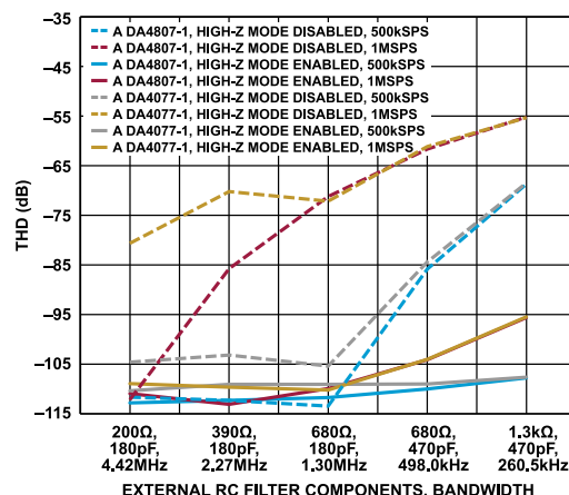
Figure 73. THD vs. External RC Filter Components, Bandwidth for Various Amplifiers ( V_{REF} = 5 V, f_{IN} = 1 kHz)
