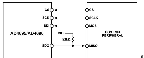
Figure 119. AD4695/AD4696 SPI Connection Diagram (Single-SDO Mode)
