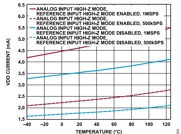
Figure 54. VDD Current vs. Temperature, Internal LDO Disabled
