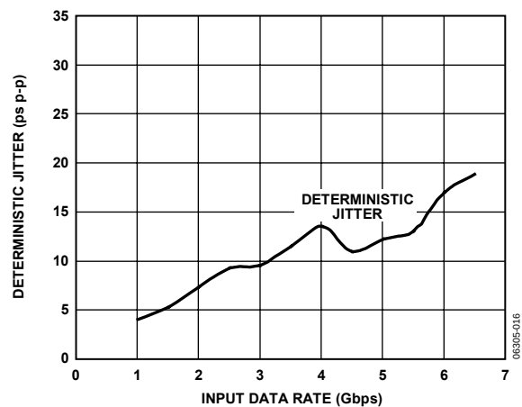
Figure 16. Deterministic Jitter vs. Data Rate (No EQ)
