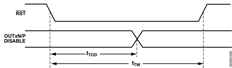
Figure 6. Asynchronous Reset
