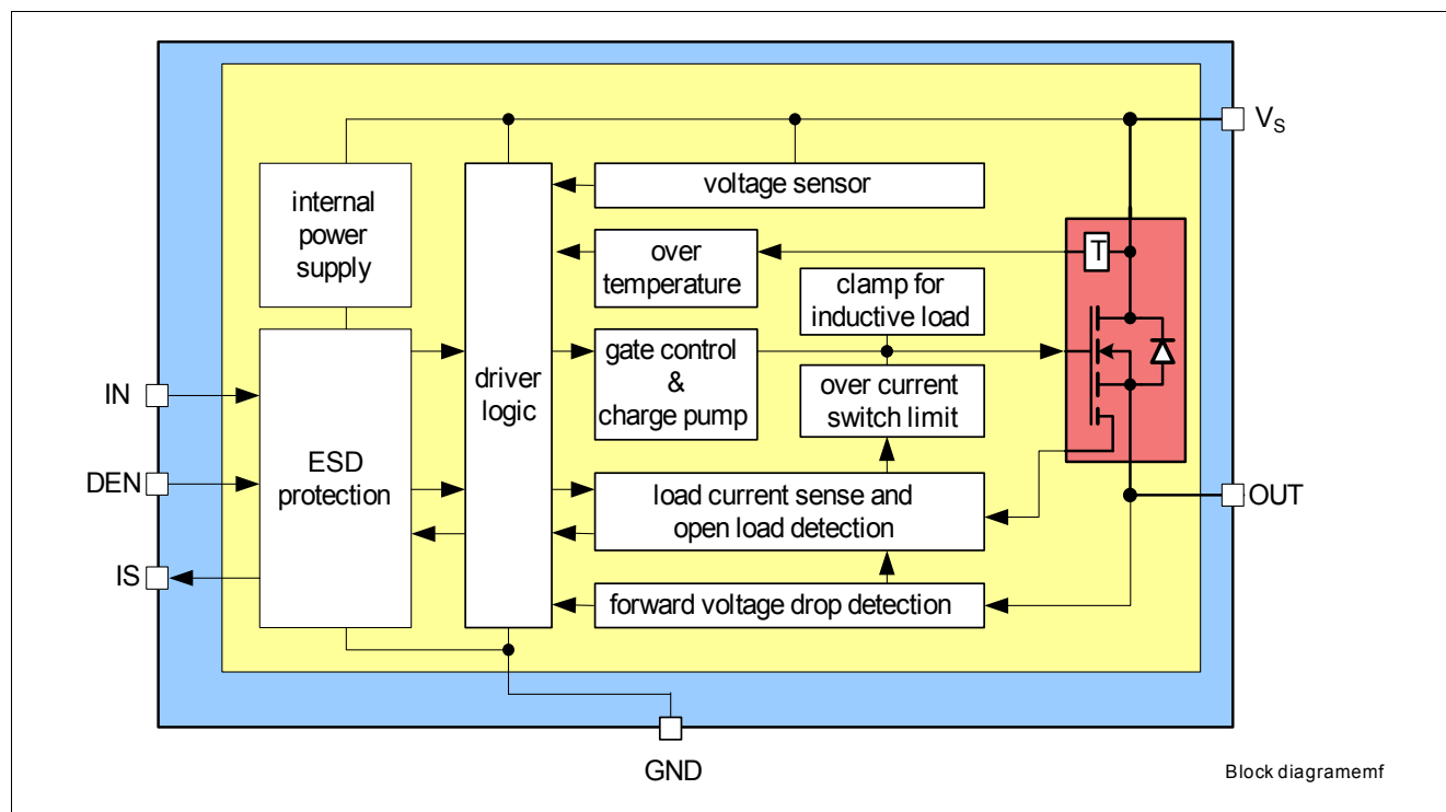
Figure 1 Block Diagram for the BTT6200-1EJA
