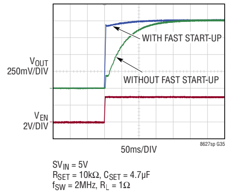
Start-Up Time with and without Fast Start-Up Circuitry for Large C_{SET}
