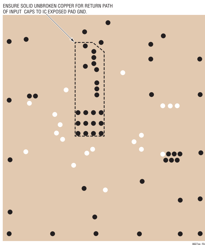
(b) Ground Plane Layer
