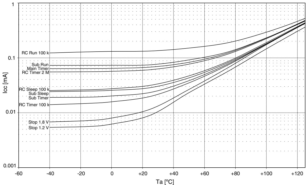
CY96F313/F315 Low power mode currents
