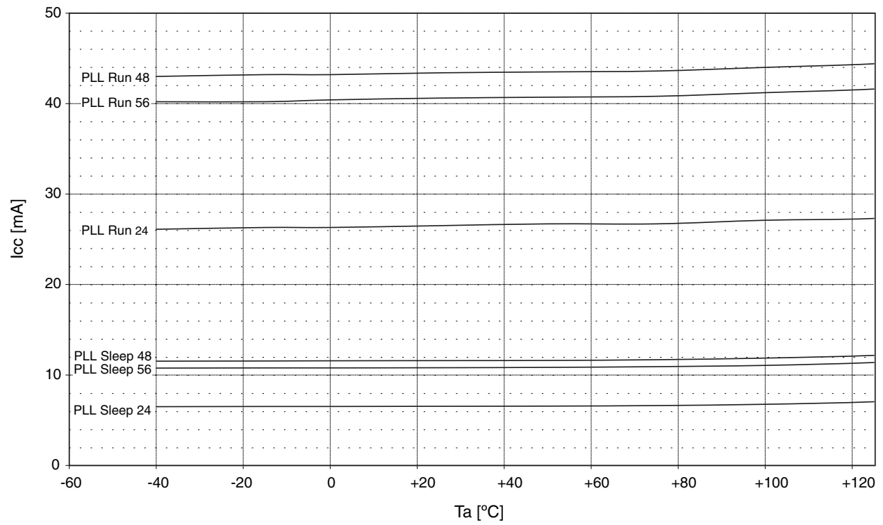
CY96F313/F315 PLL Run and Sleep mode currents
