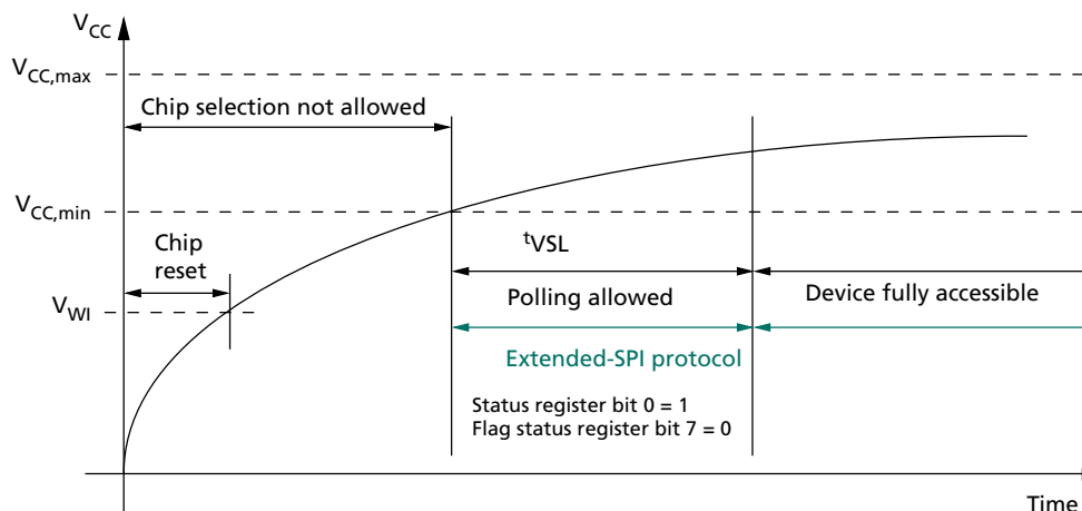
Figure 43: Power-Up Timing
