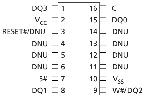
Figure 5: 16-Pin, Plastic Small Outline – SO16 (Top View)
