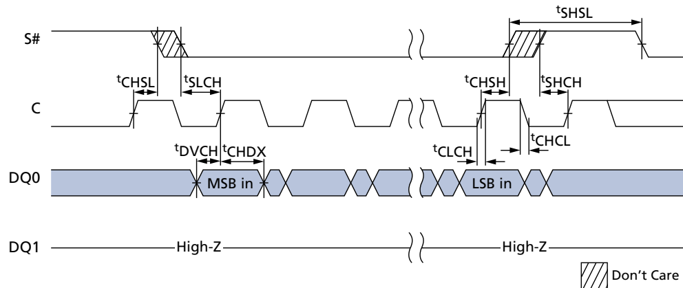
Figure 47: Serial Input Timing
