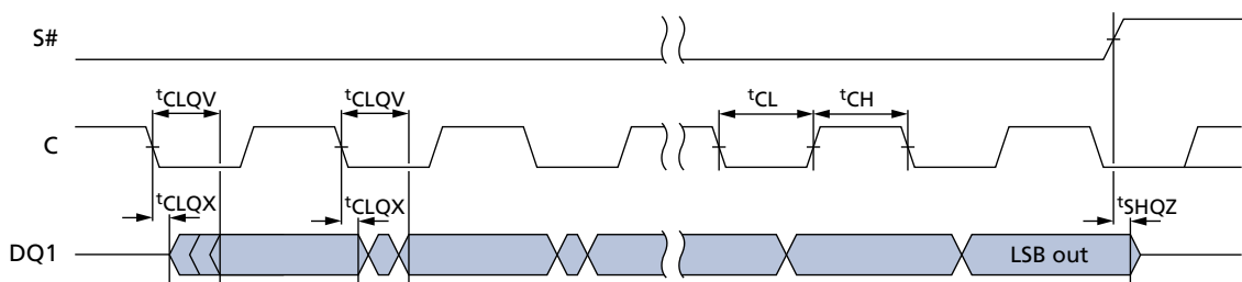
Figure 50: Output Timing
