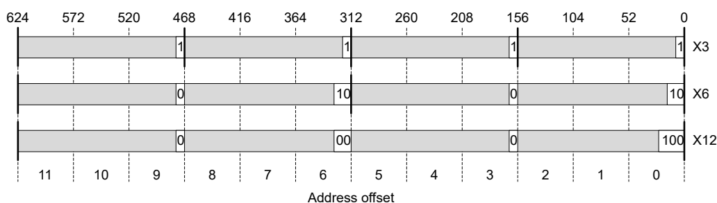
Figure 4-22. VCAP ES2 Entry Type-Group Fields
