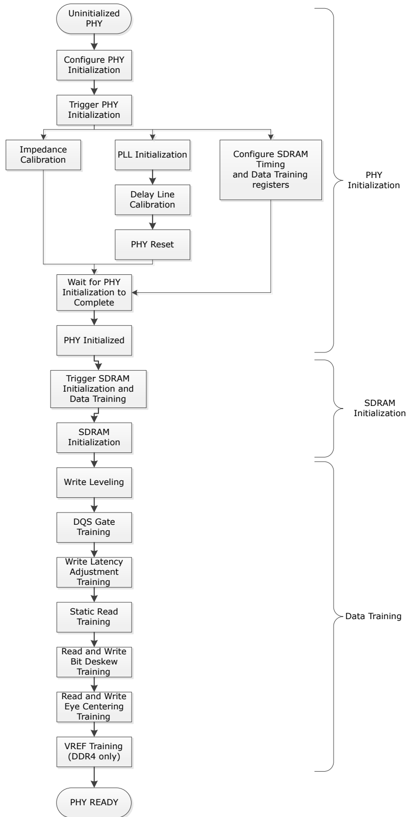
Figure 5-11. PHY Initialization Flow
