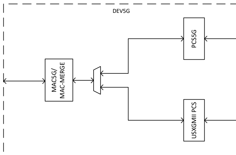
Figure 4-9. DEV10G Port Module
