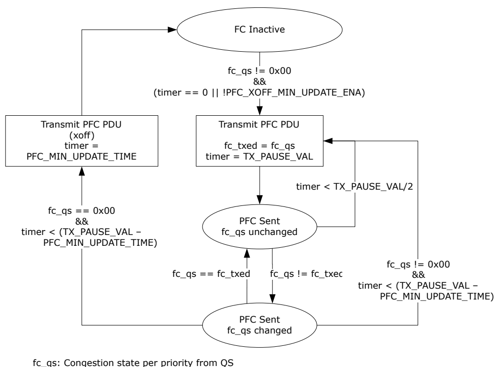
Figure 4-98. PFC Generation per Port
