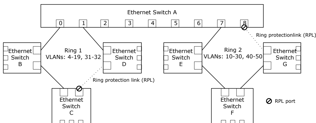
Figure 4-99. Ethernet Ring Protection Example
