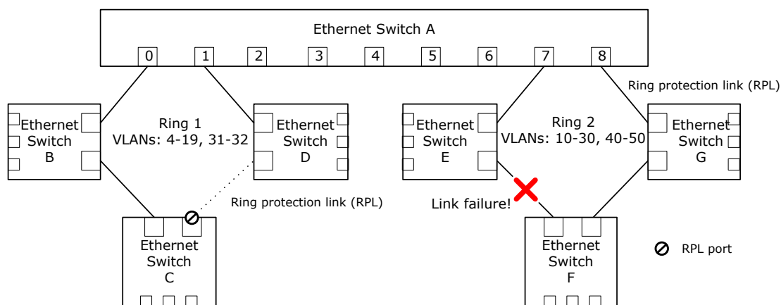
Figure 4-100. Ethernet Ring with Failure
