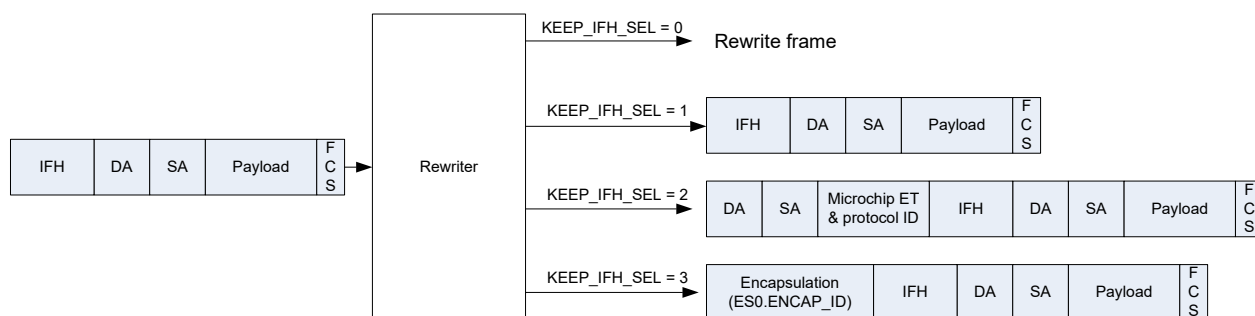
Figure 4-96. Supported KEEP_IFH_SEL Formats
