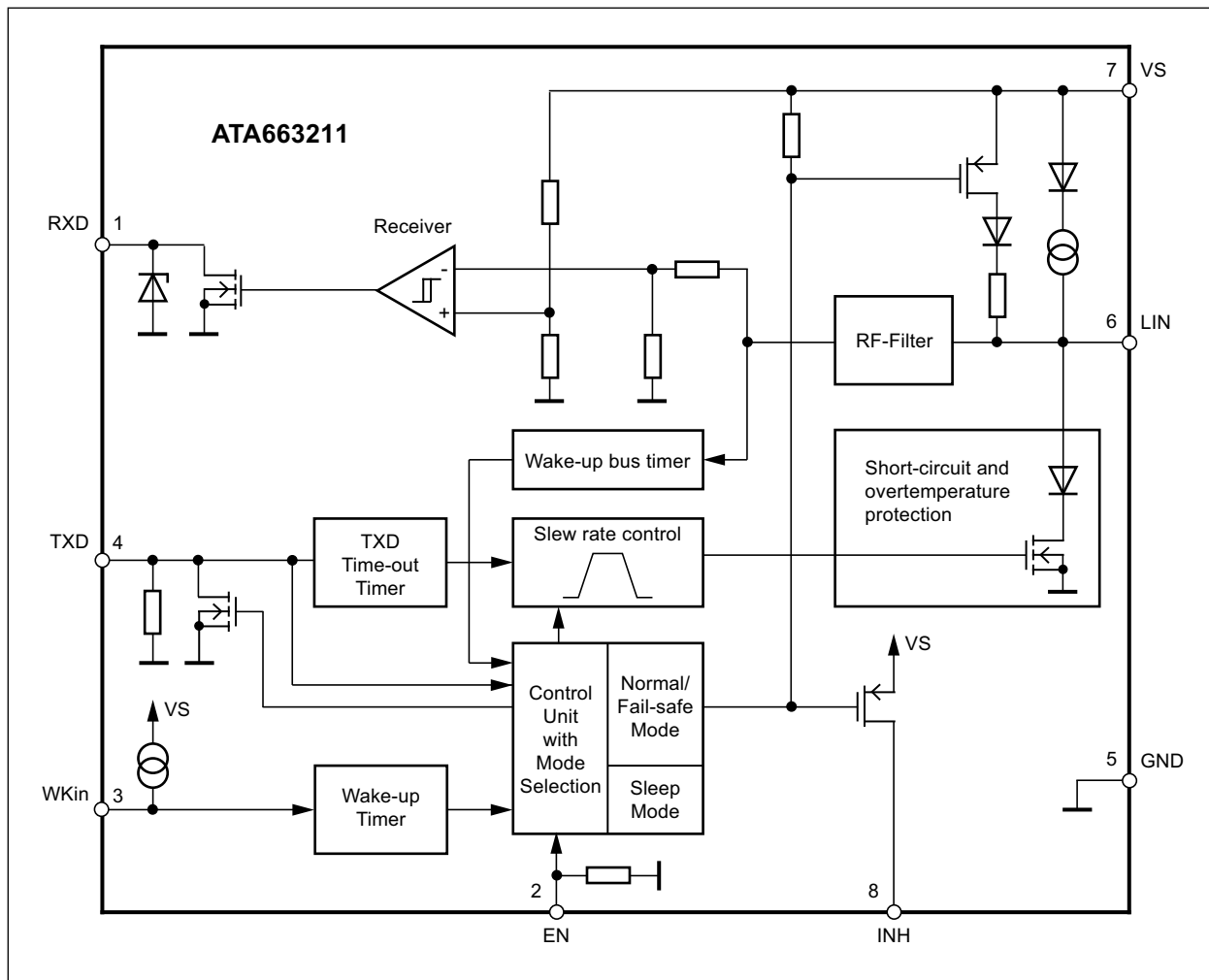
ATA663211 Block Diagram
