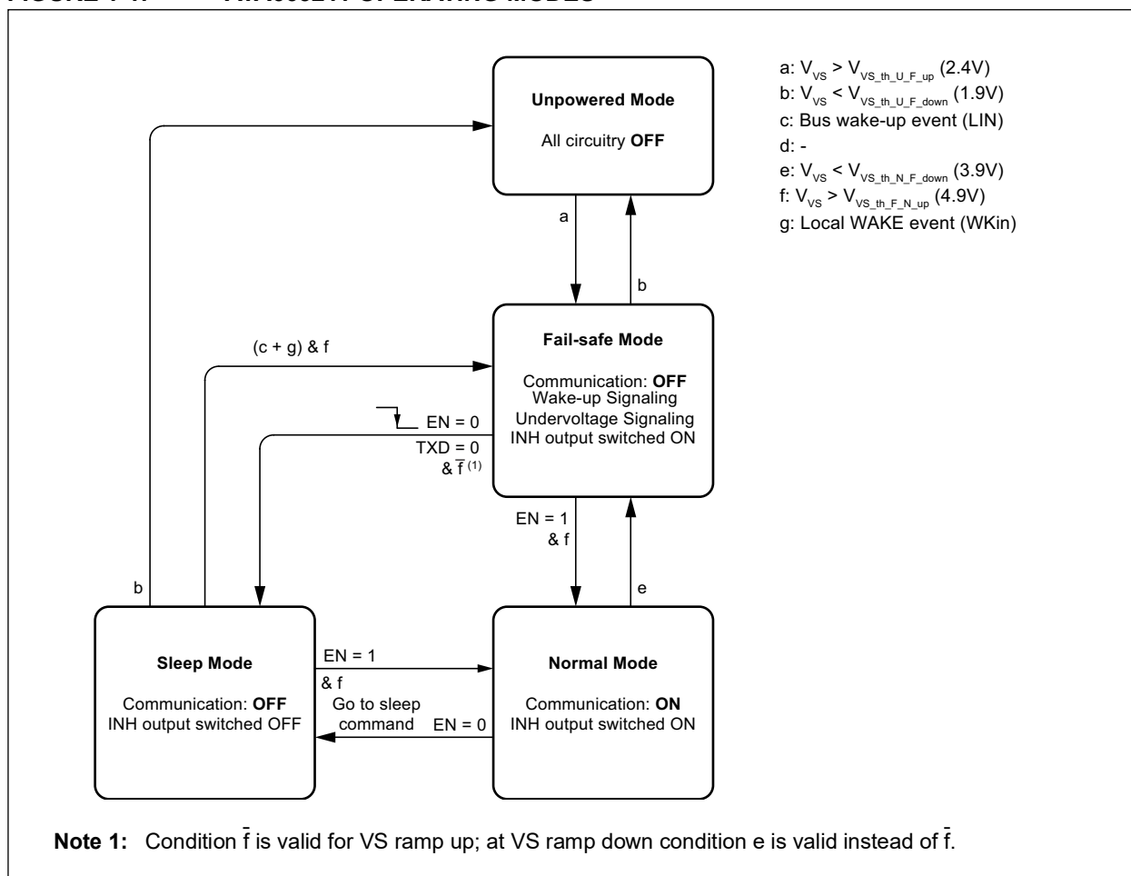
FIGURE 1-1: ATA663211 OPERATING MODES
