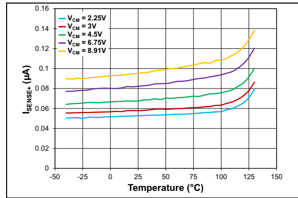
FIGURE 2-28: I_{SENSE+} vs. T_A , Common Mode, Multiple V_{CM} .
