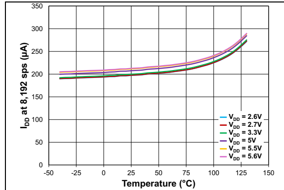
FIGURE 2-23: I_{DD} at 8,192 sps vs. T_A , Multiple V_{DD} .
