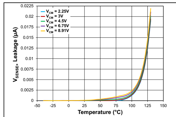
FIGURE 2-30: V_{SENSE+} Leakage vs. T_A , Common Mode, Multiple V_{CM} .
