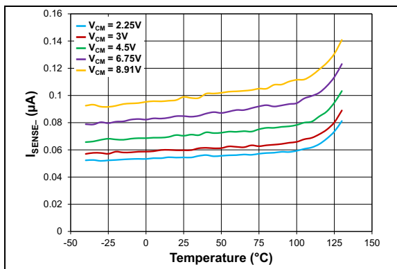
FIGURE 2-27: I_{SENSE-} vs. T_A , Common Mode, Multiple V_{CM} .
