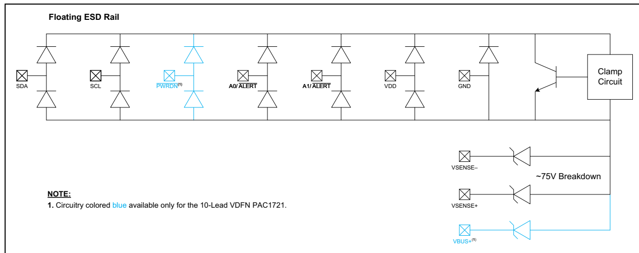
FIGURE 1-1: PAC1721 ESD Protection Circuitry.
