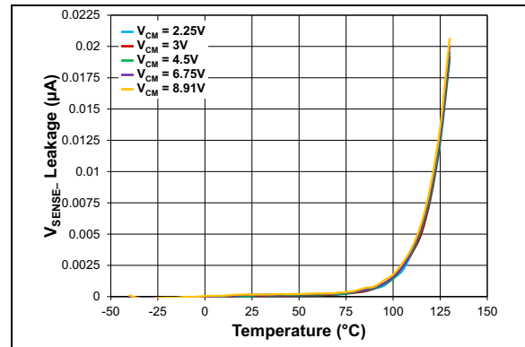
FIGURE 2-29: V_{SENSE-} Leakage vs. T_A , Common Mode, Multiple V_{CM} .
