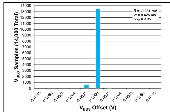
FIGURE 2-18: V_{BUS} Zero Input Histogram, Bipolar FSR/2 Mode, n = 14,000 Total Samples, 8x Average.
