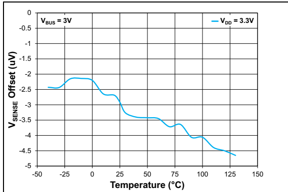
FIGURE 2-20: V_{SENSE} Offset vs. T_A , V_{DD} = 3.3\text{V} , V_{BUS} = 3.0\text{V} , Bipolar FSR Mode.
