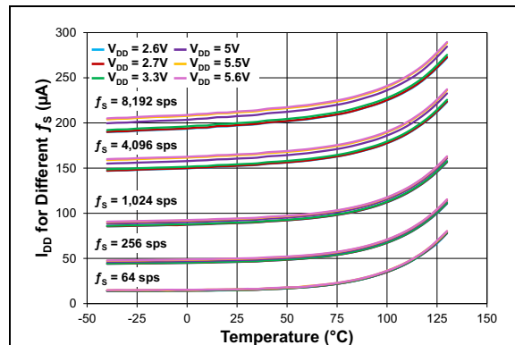
FIGURE 2-24: I_{DD} vs. T_A , Multiple V_{DD} , Multiple Sample Rates ( f_s ).
