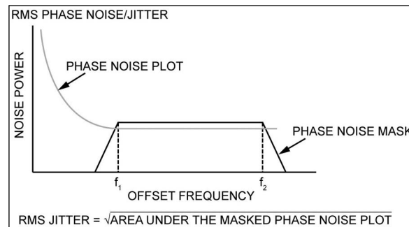
FIGURE 5-5: RMS Phase/Noise/Jitter.
