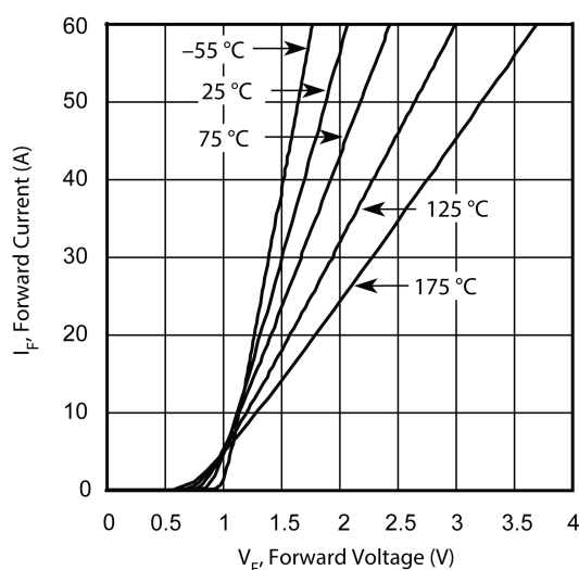
Figure 1-1. Forward Current vs. Forward Voltage
