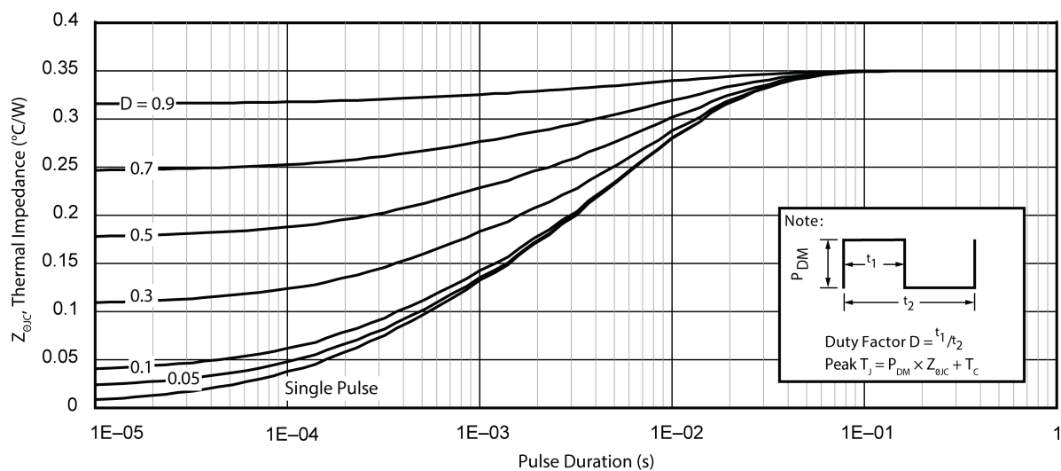
Figure 1-7. Maximum Transient Thermal Impedance
