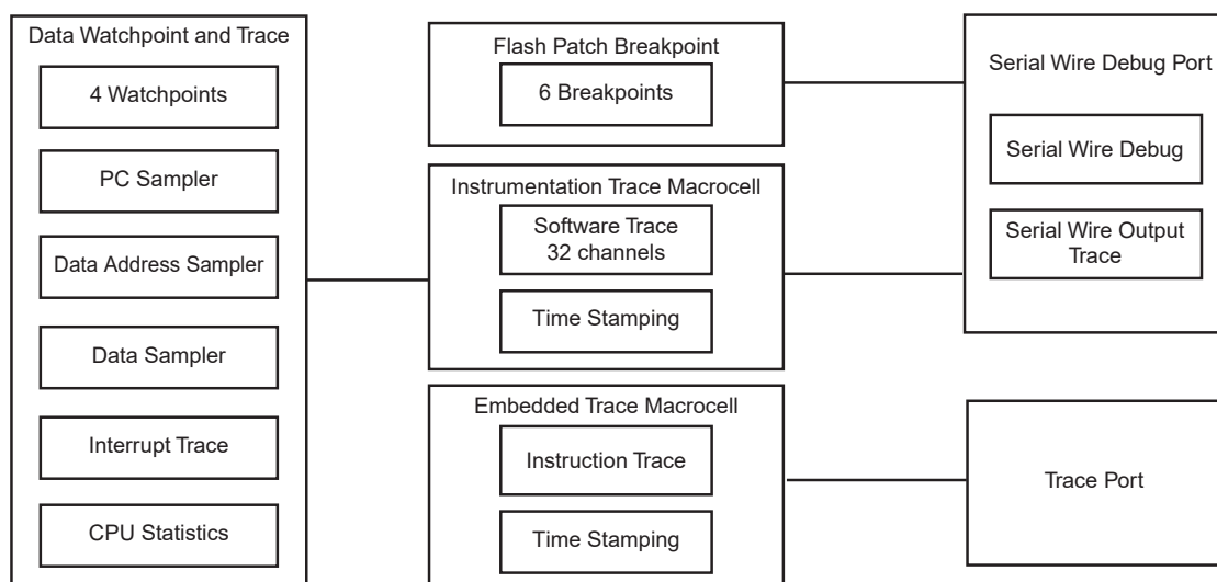
Figure 16-4. Debug Architecture
