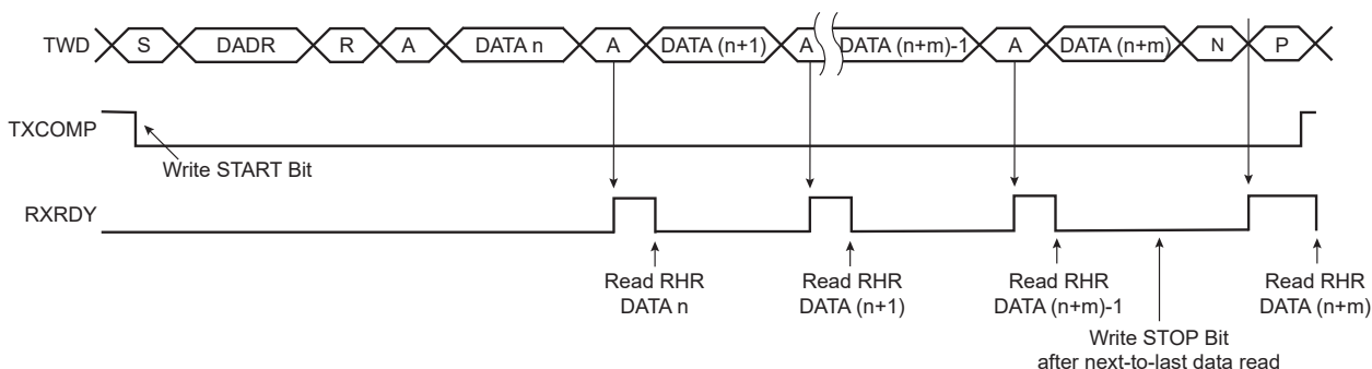
Figure 43-9. Master Read Clock Stretching with Multiple Data Bytes
