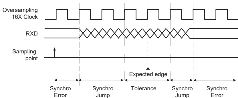
Figure 46-10. Bit Resynchronization
