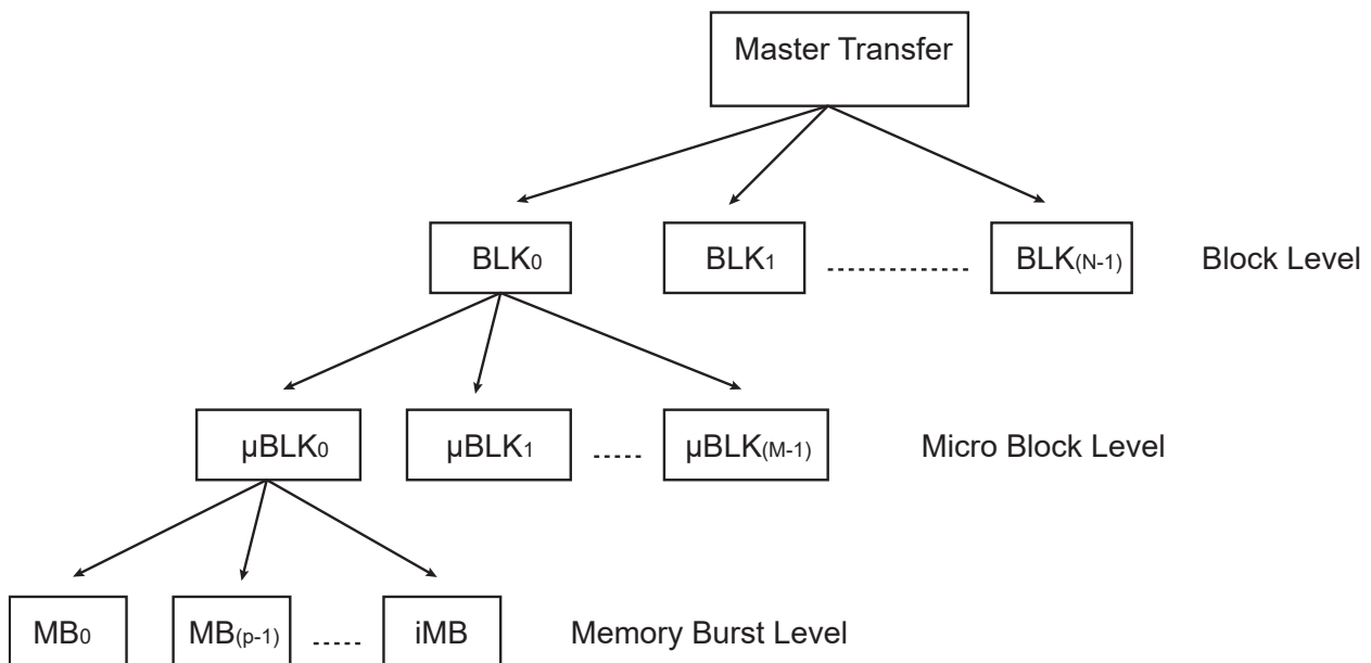
Figure 36-2. XDMAC Memory Transfer Hierarchy
