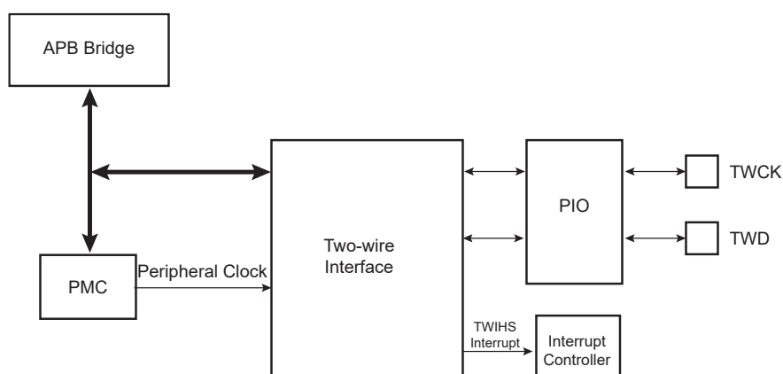
Figure 43-1. Block Diagram
