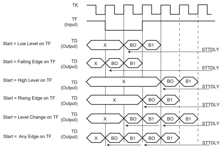
Figure 44-13. Transmit Start Mode
