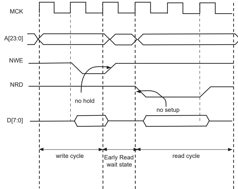
Figure 35-18. Early Read Wait State: Write with No Hold Followed by Read with No Setup
