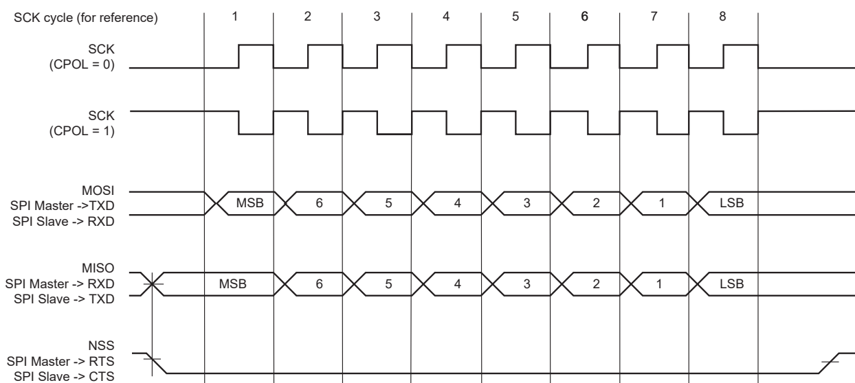
Figure 46-37. SPI Transfer Format (CPHA = 1, 8 bits per transfer)
