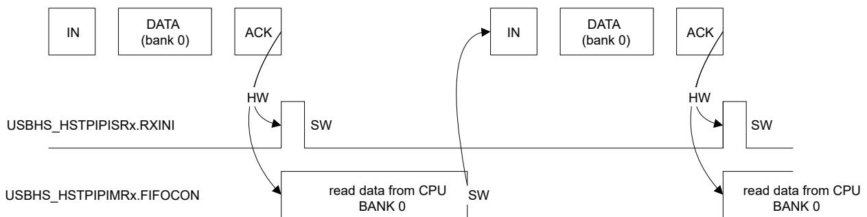
Figure 39-19. Example of an IN Pipe with one Data Bank
