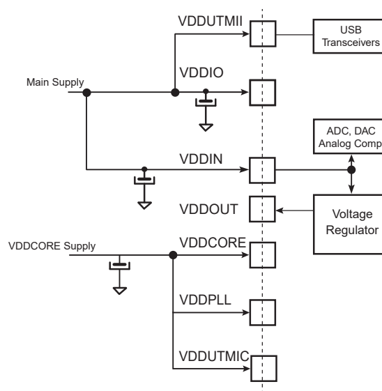
Figure 23-2. Separate Backup Supply Powering Scheme
