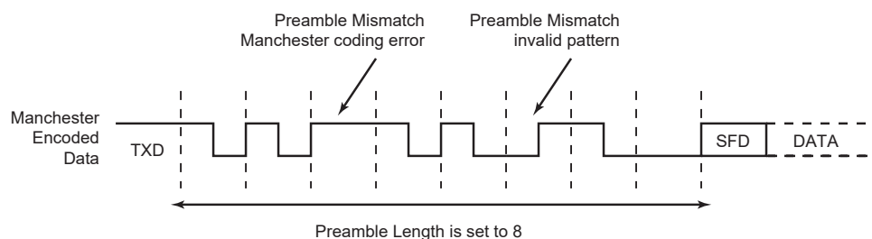
Figure 46-14. Preamble Pattern Mismatch
