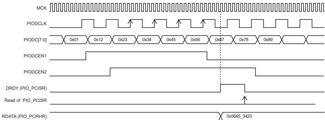
Figure 32-10. Parallel Capture Mode Waveforms (DSIZE = 2, ALWYS = 0, HALFS = 0)
