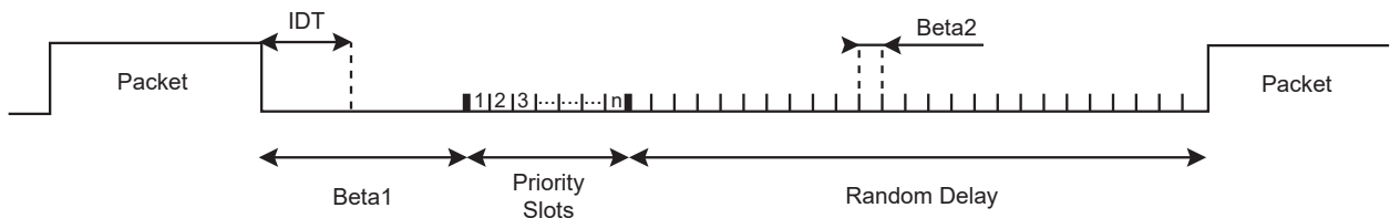
Figure 46-59. LON Timings
