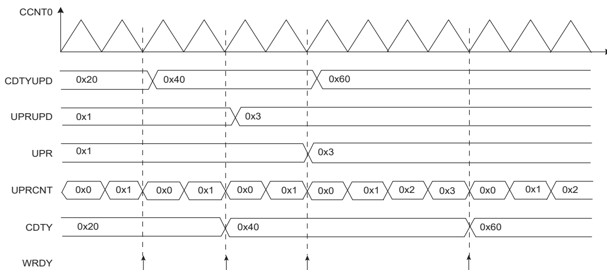
Figure 51-20. Method 2 (UPDM = 1)
