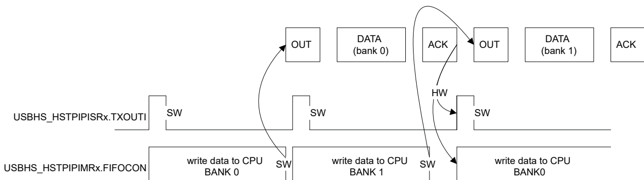
Figure 39-23. Example of an OUT Pipe with two Data Banks and a Bank Switching Delay
