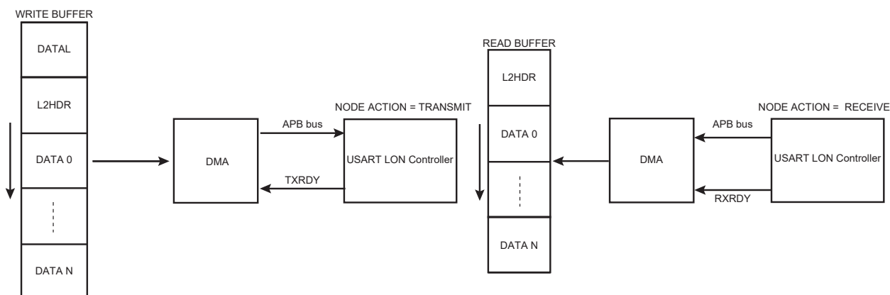
Figure 46-63. DMAM = 1
