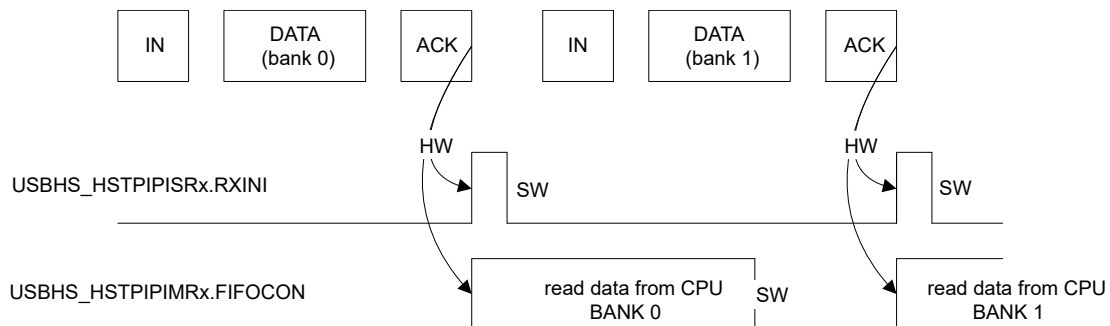
Figure 39-20. Example of an IN Pipe with two Data Banks
