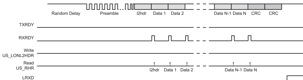
Figure 46-62. Rx Frame
