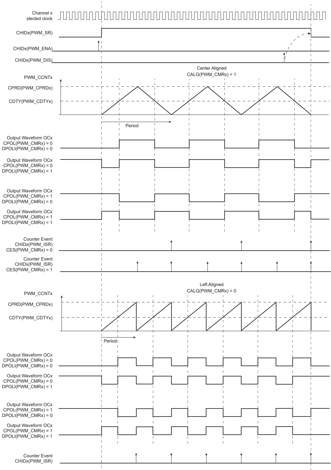
Figure 51-5. Waveform Properties
