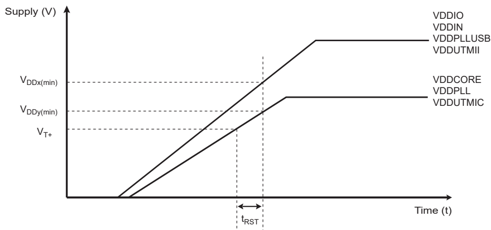
Figure 7-1. Powerup Sequence
