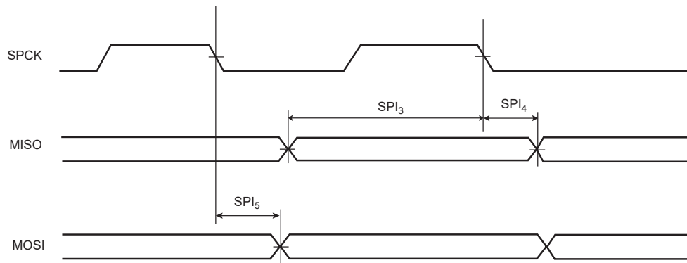
Figure 58-22. SPI Slave Mode with (CPOL=0 and NCPHA=1) or (CPOL=1 and NCPHA=0)
