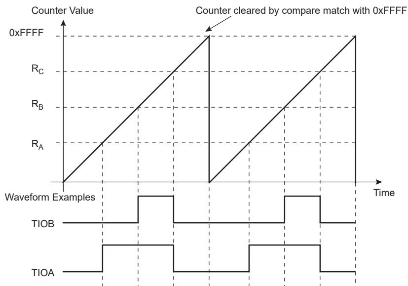
Figure 50-8. WAVSEL = 00 without Trigger
