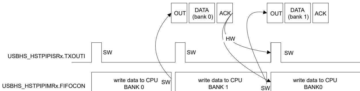
Figure 39-22. Example of an OUT Pipe with two Data Banks and no Bank Switching Delay
