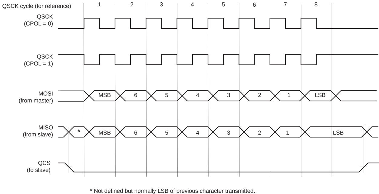
Figure 42-3. QSPI Transfer Format (QSPI_SCR.CPHA = 1, 8 bits per transfer)
