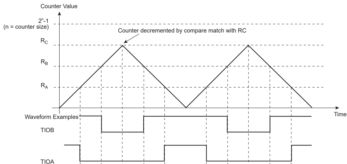
Figure 50-14. WAVSEL = 11 without Trigger
