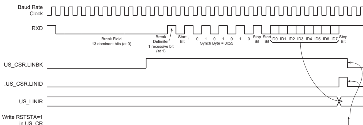
Figure 46-40. Header Reception
