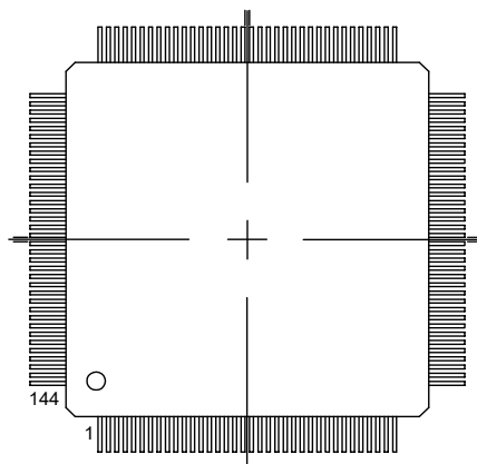
Figure 6-2. Orientation of the 144-pin LQFP Package
