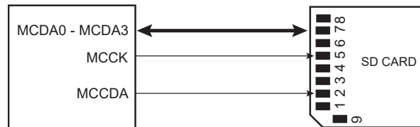
Figure 40-6. SD Card Bus Connections with One Slot
