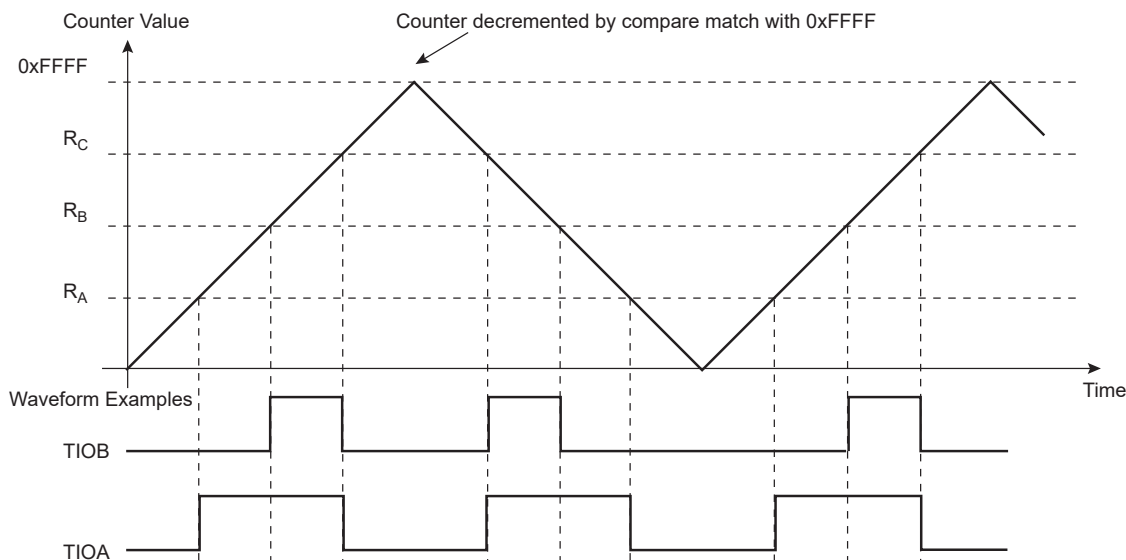
Figure 50-12. WAVSEL = 01 without Trigger
