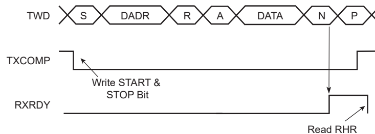
Figure 43-7. Master Read with One Data Byte
