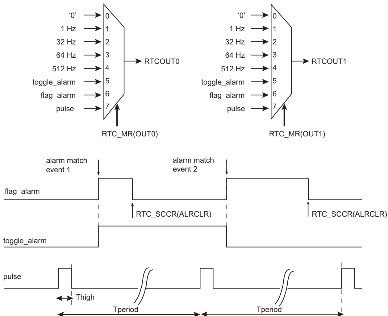
Figure 27-6. Waveform Generation
