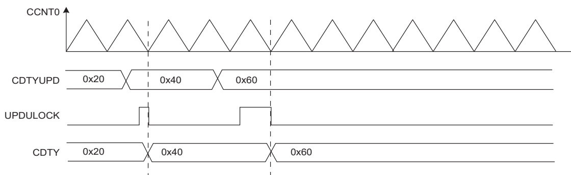
Figure 51-19. Method 1 (UPDM = 0)
