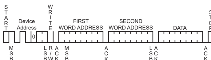
Figure 43-12. Internal Address Usage
