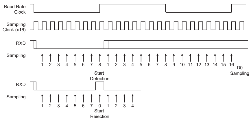
Figure 46-11. Asynchronous Start Detection
