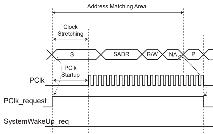
Figure 43-40. No Address Match (Data Matching Disabled)
