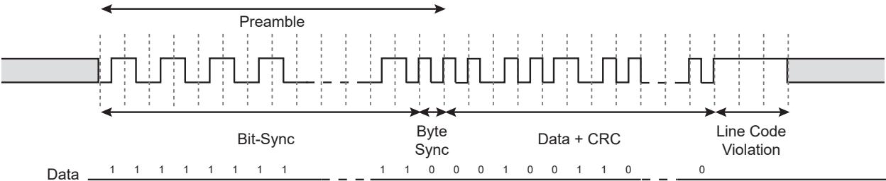
Figure 46-55. LON Framing
