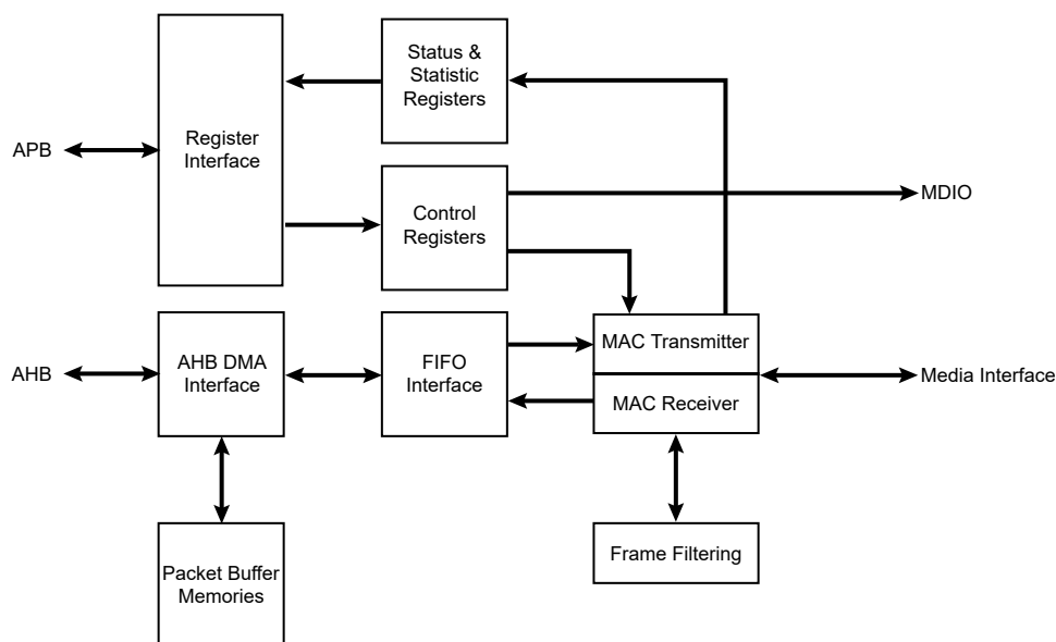
Figure 38-1. Block Diagram
