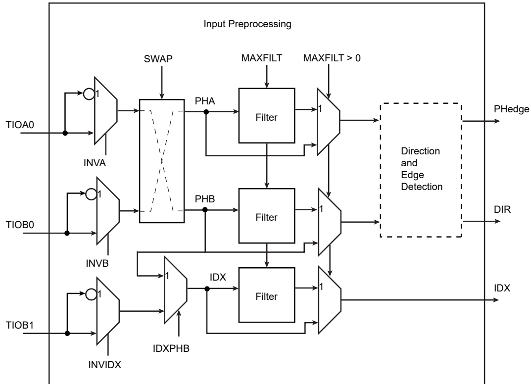
Figure 50-18. Input Stage
