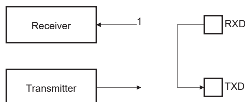
Figure 46-69. Remote Loopback Mode Configuration
