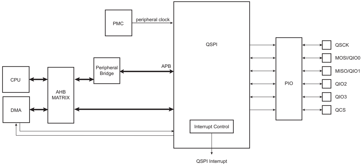
Figure 42-1. Block Diagram
