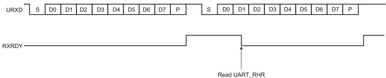
Figure 47-5. Receiver Ready
