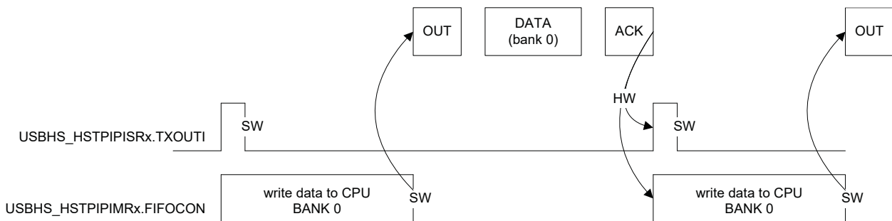
Figure 39-21. Example of an OUT Pipe with one Data Bank
