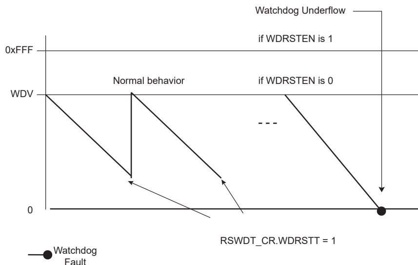
Figure 25-2. Watchdog Behavior
