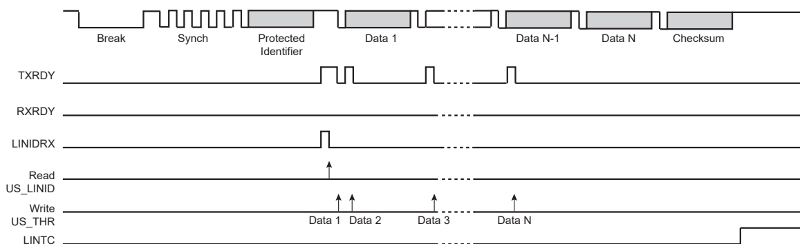
Figure 46-48. Slave Node Configuration, NACT = PUBLISH
