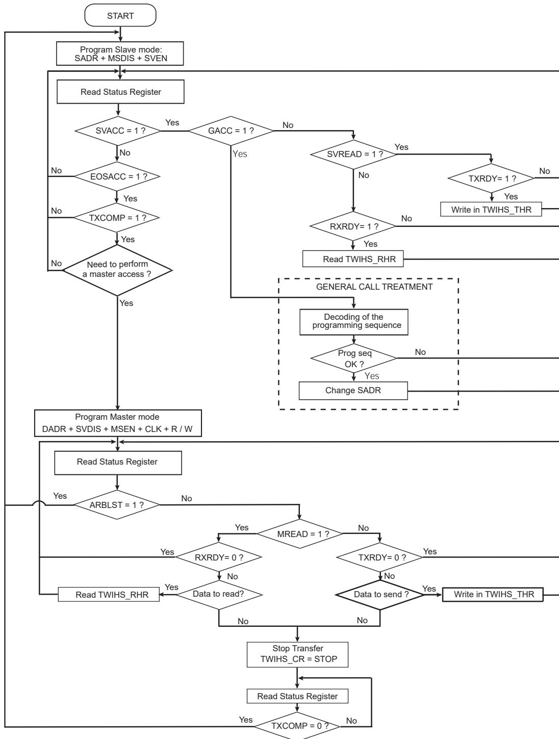
Figure 43-30. Multimaster Flowchart
