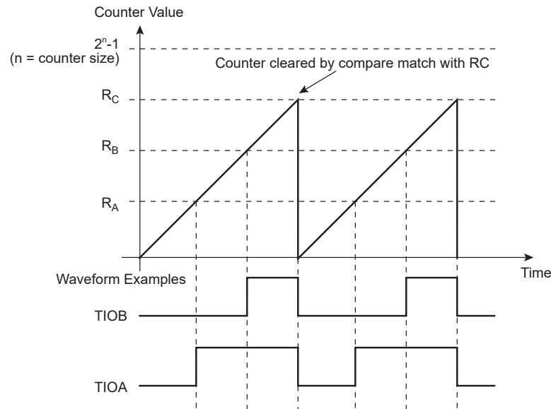
Figure 50-10. WAVSEL = 10 without Trigger
