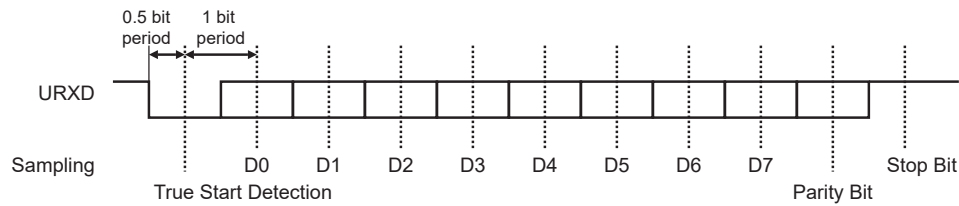
Figure 47-4. Character Reception
