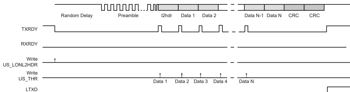
Figure 46-61. Tx Frame
