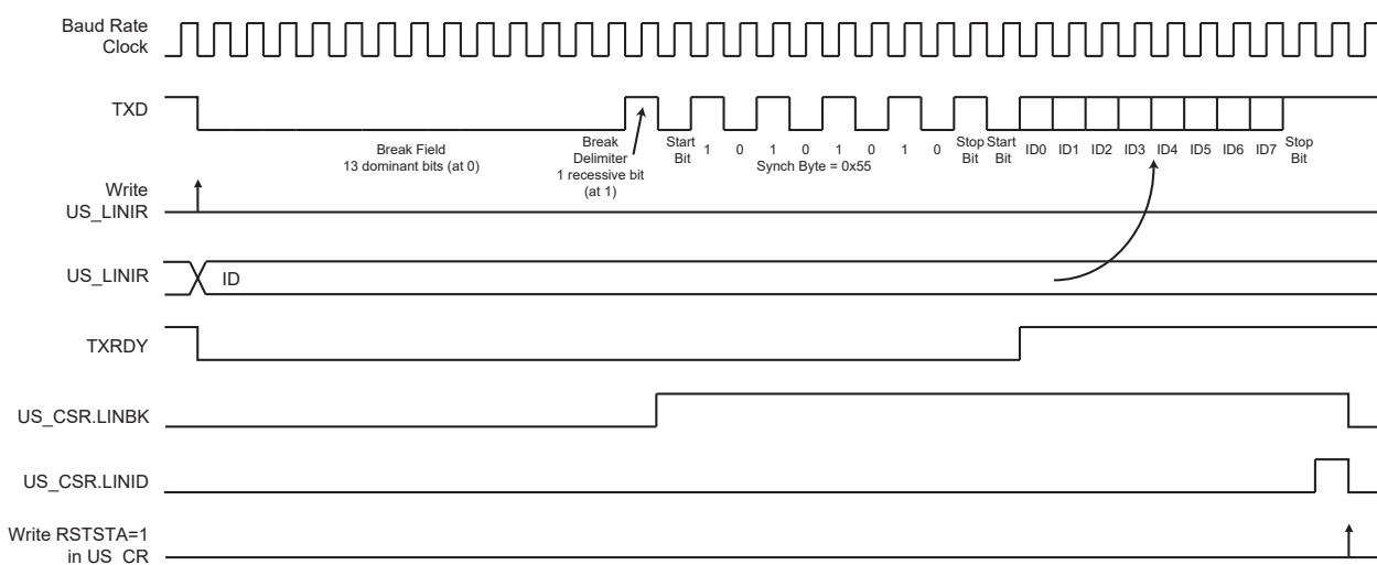
Figure 46-39. Header Transmission
