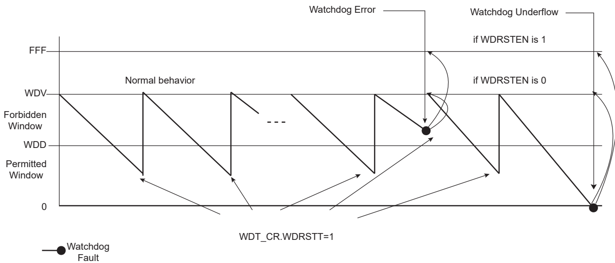
Figure 24-2. Watchdog Behavior
