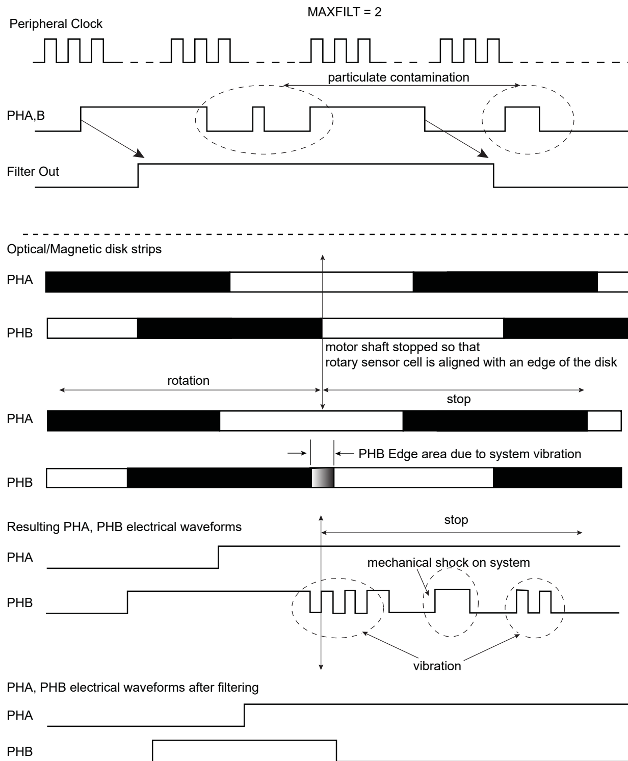
Figure 50-19. Filtering Examples
