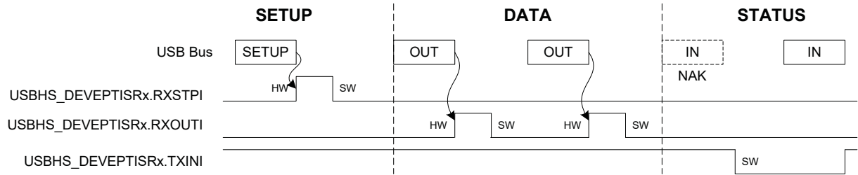
Figure 39-9. Control Write
