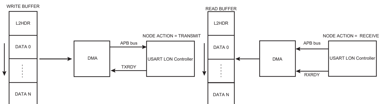
Figure 46-64. DMAM = 0
