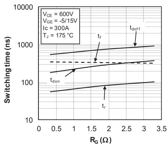
Figure 1-7. Switching Time vs. Gate Resistance
