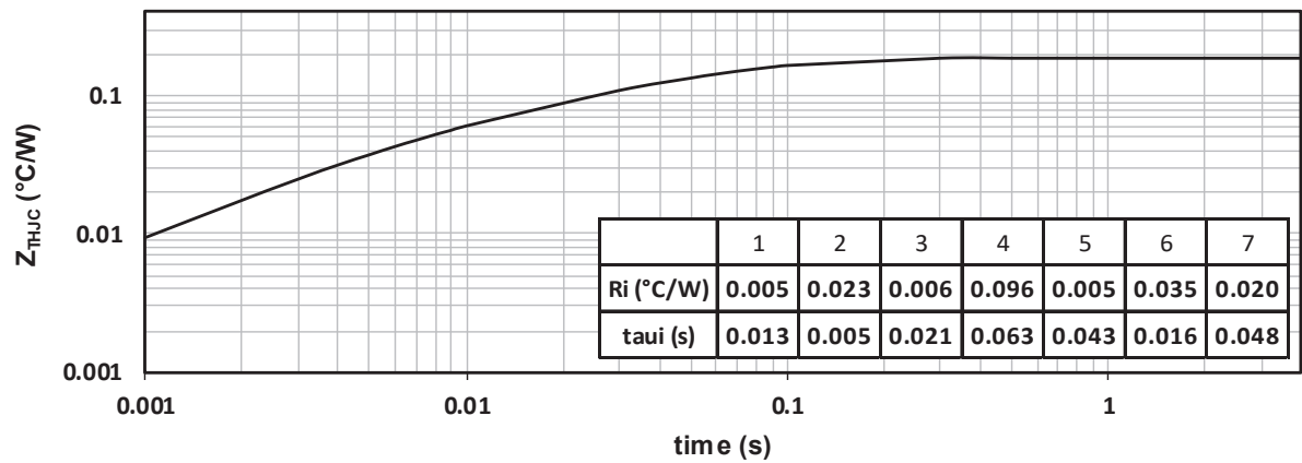
Figure 1-11. Maximum Thermal Impedance
