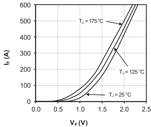
Figure 1-12. Forward Characteristics
