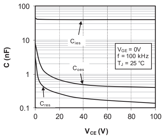
Figure 1-9. Capacity Characteristics
