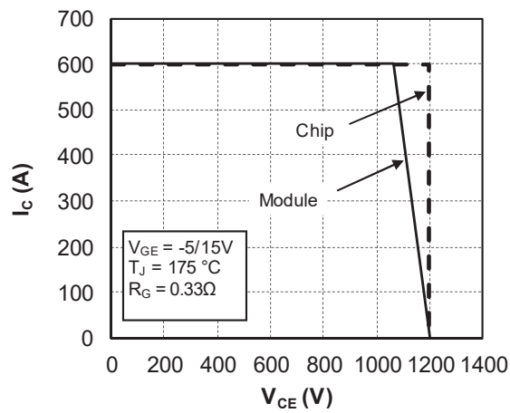
Figure 1-10. Reverse Bias Safe Operating Area
