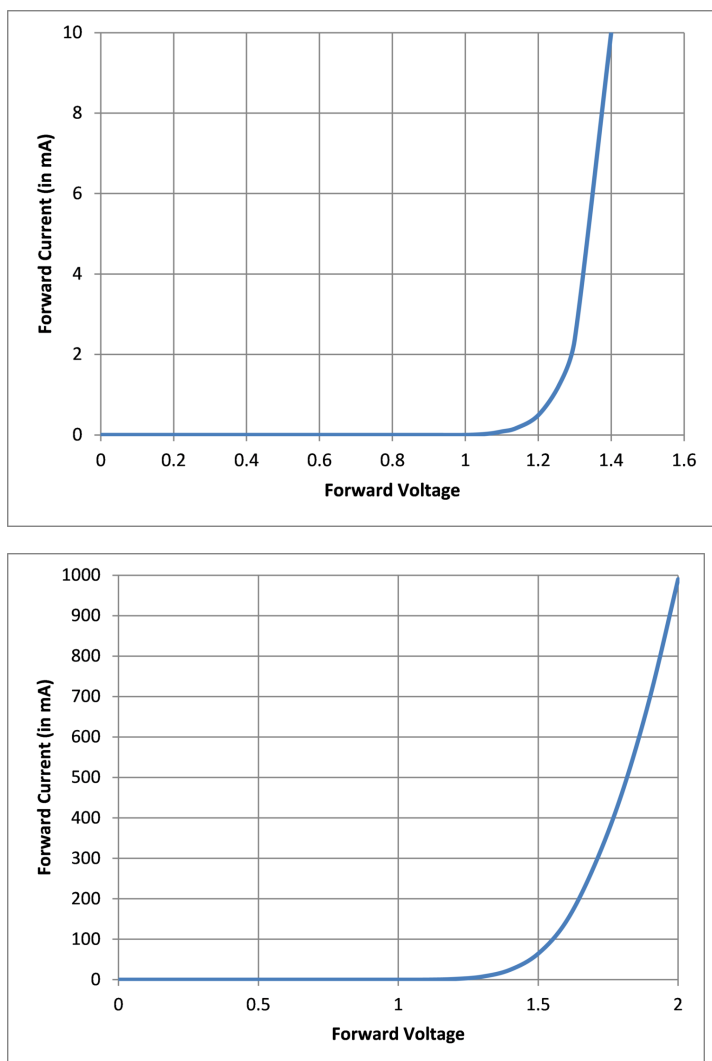
Figure 7-1. Forward Characteristics, 0 to 10 mA and 0 to 1000 mA, Measured A to K (Two Diodes in Series)
