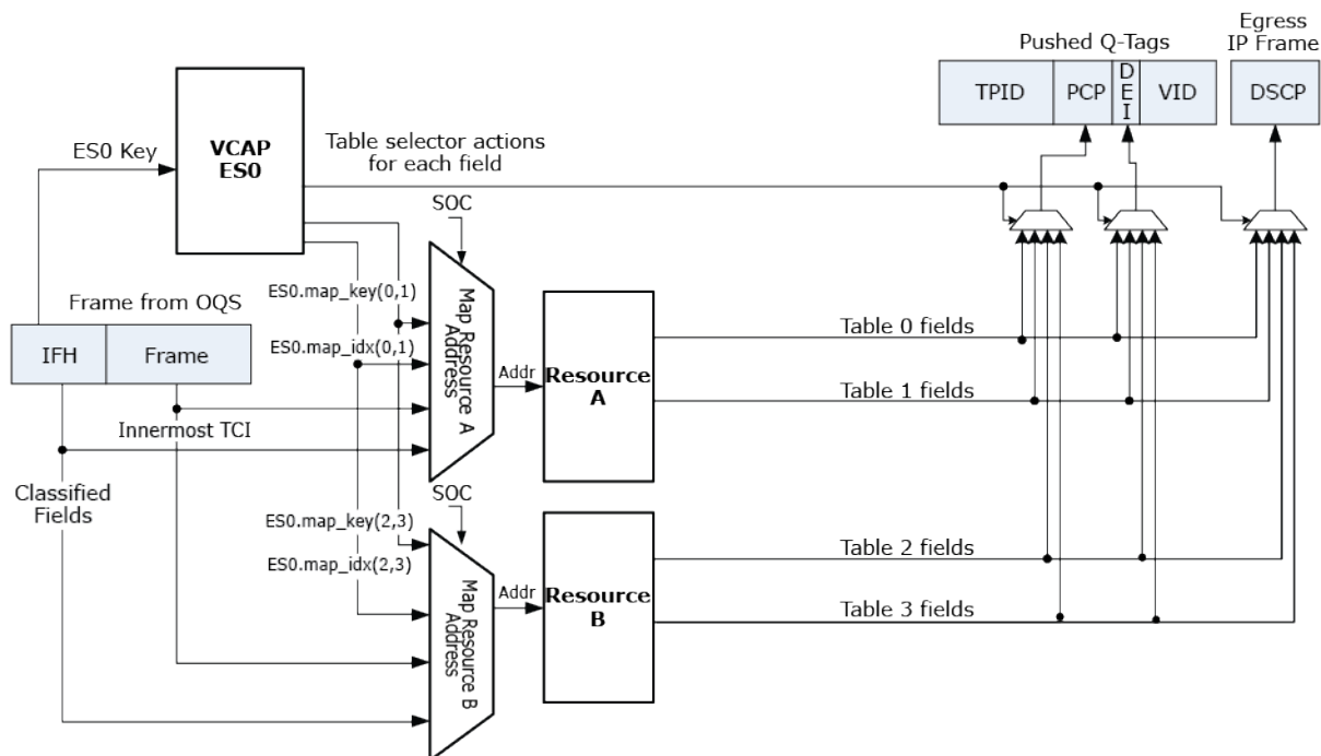
Figure 4-92. Mapping Tables
