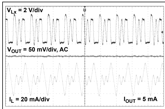
FIGURE 2-25: PWM Light Load Switching Waveforms (MCP1603B).
