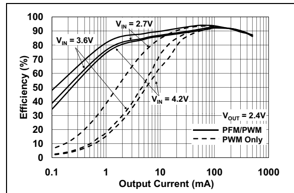
FIGURE 2-12: PFM/PWM Efficiency vs. Output Load ( V_{OUT} = 2.4\text{V} ).
