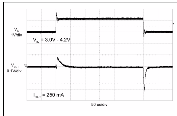
FIGURE 2-24: Output Voltage Line Step Response vs. Time.
