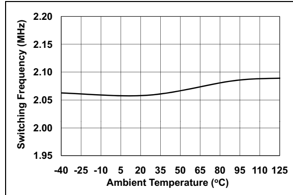
FIGURE 2-16: Switching Frequency vs. Ambient Temperature.
