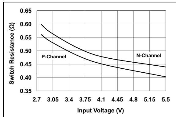
FIGURE 2-18: Switch Resistance vs. Input Voltage.
