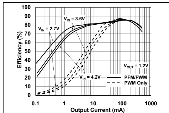
FIGURE 2-6: Efficiency vs. Output Load ( V_{OUT} = 1.2V ).
