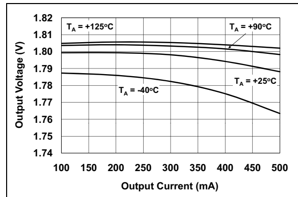
FIGURE 2-11: Output Voltage vs. Load Current ( V_{OUT} = 1.8\text{V} ).
