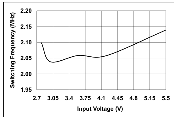
FIGURE 2-17: Switching Frequency vs. Input Voltage.
