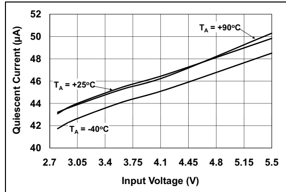
FIGURE 2-4: PFM I_Q vs. Input Voltage (MCP1603/L).
