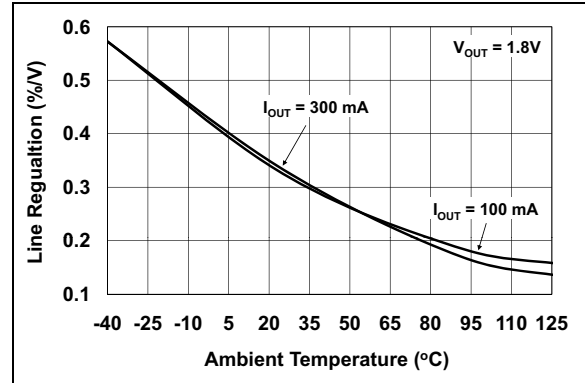
FIGURE 2-10: Line Regulation vs. Ambient Temperature ( V_{OUT} = 1.8\text{V} ).
