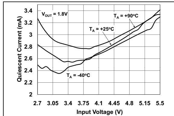
FIGURE 2-5: PWM I_Q vs. Input Voltage (MCP1603B).
