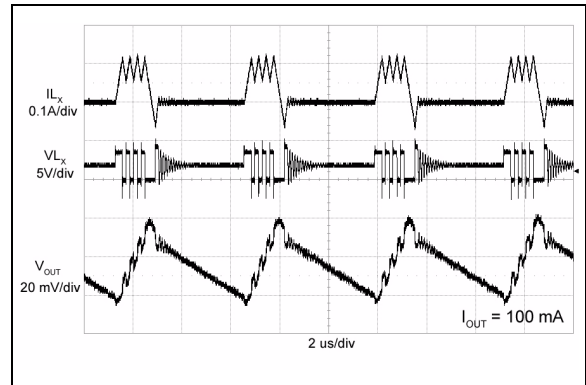
FIGURE 2-22: PFM Light Load Switching Waveforms (MCP1603/L).
