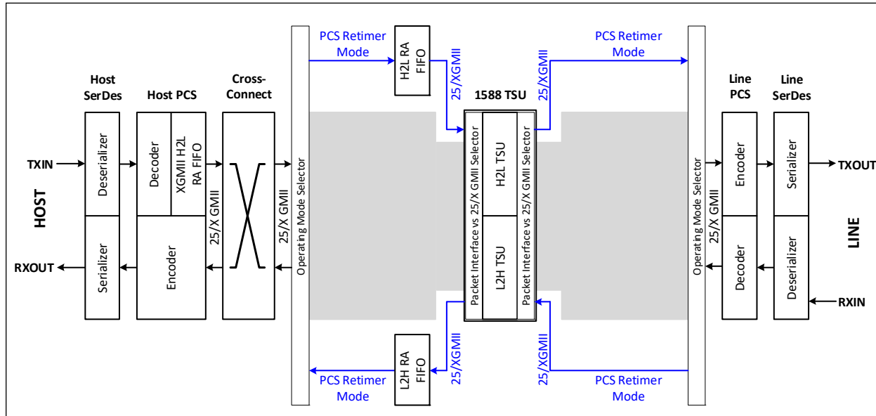
FIGURE 3-2: ETHERNET PHY, PCS RETIMER MODE DATA PATH
