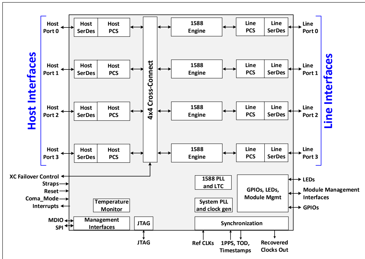
FIGURE 1-1: LAN8043 INTERNAL BLOCK DIAGRAM
