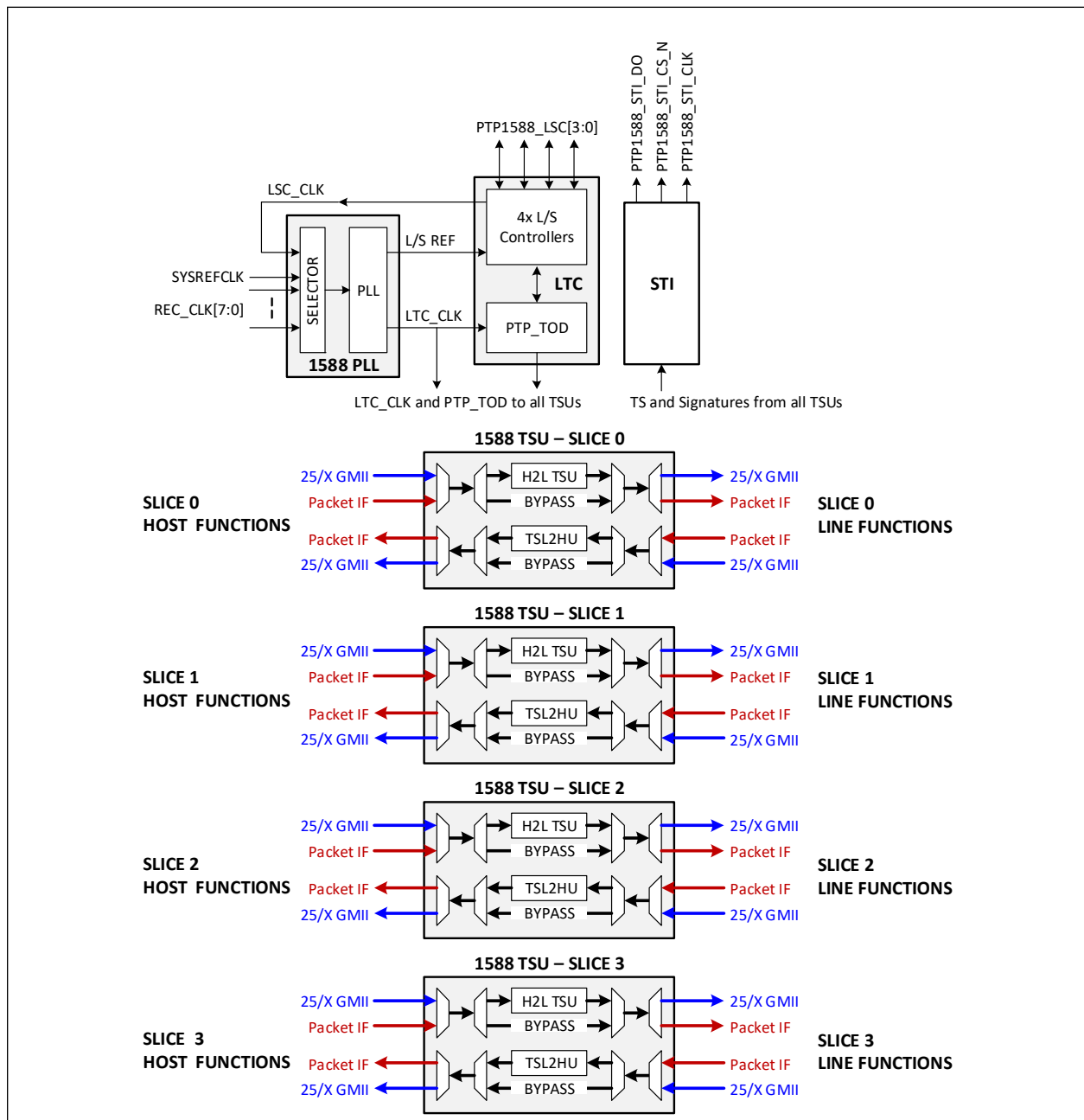
FIGURE 3-13: 1588 BLOCK DIAGRAM
