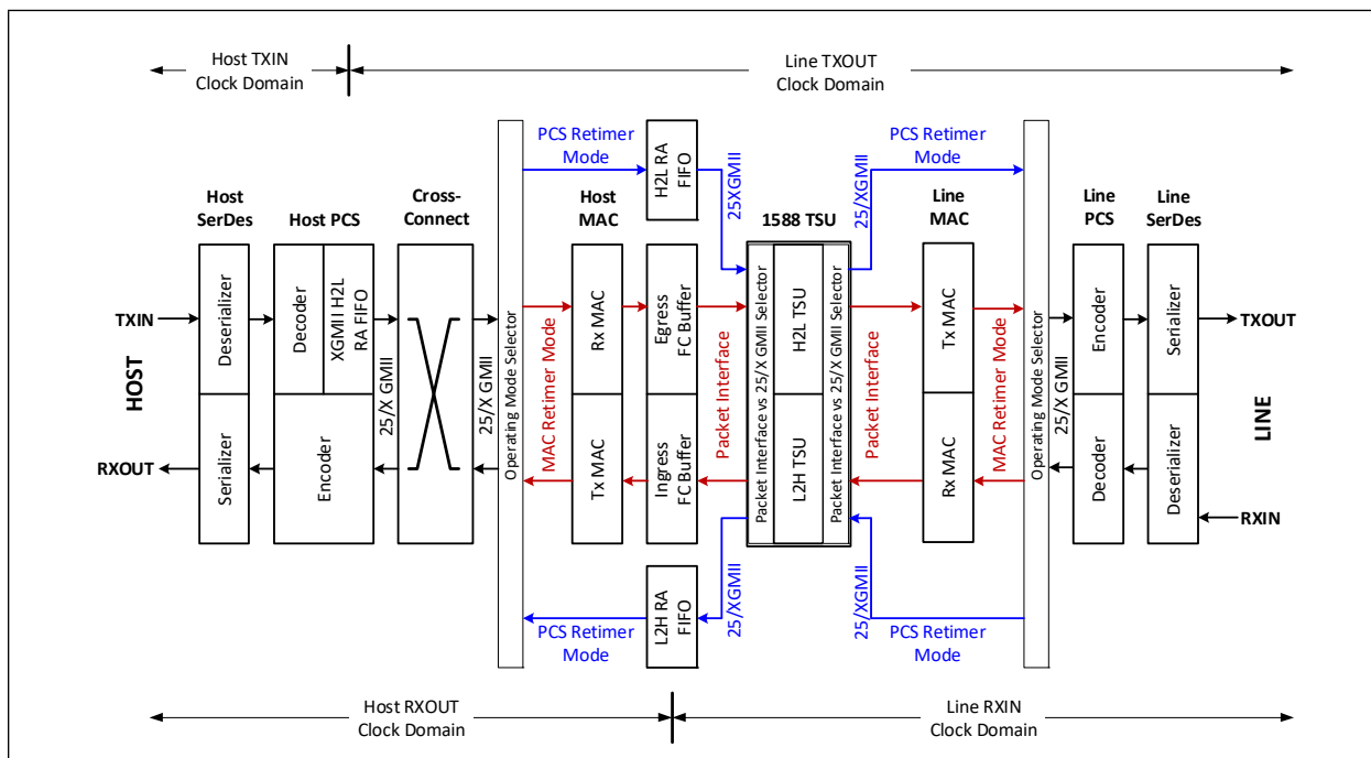
FIGURE 3-1: LAN8043 DATA PATH
