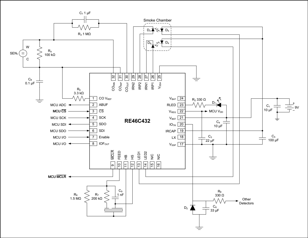
FIGURE 4-12: RE46C432 Typical 9V Battery-Only Application.
