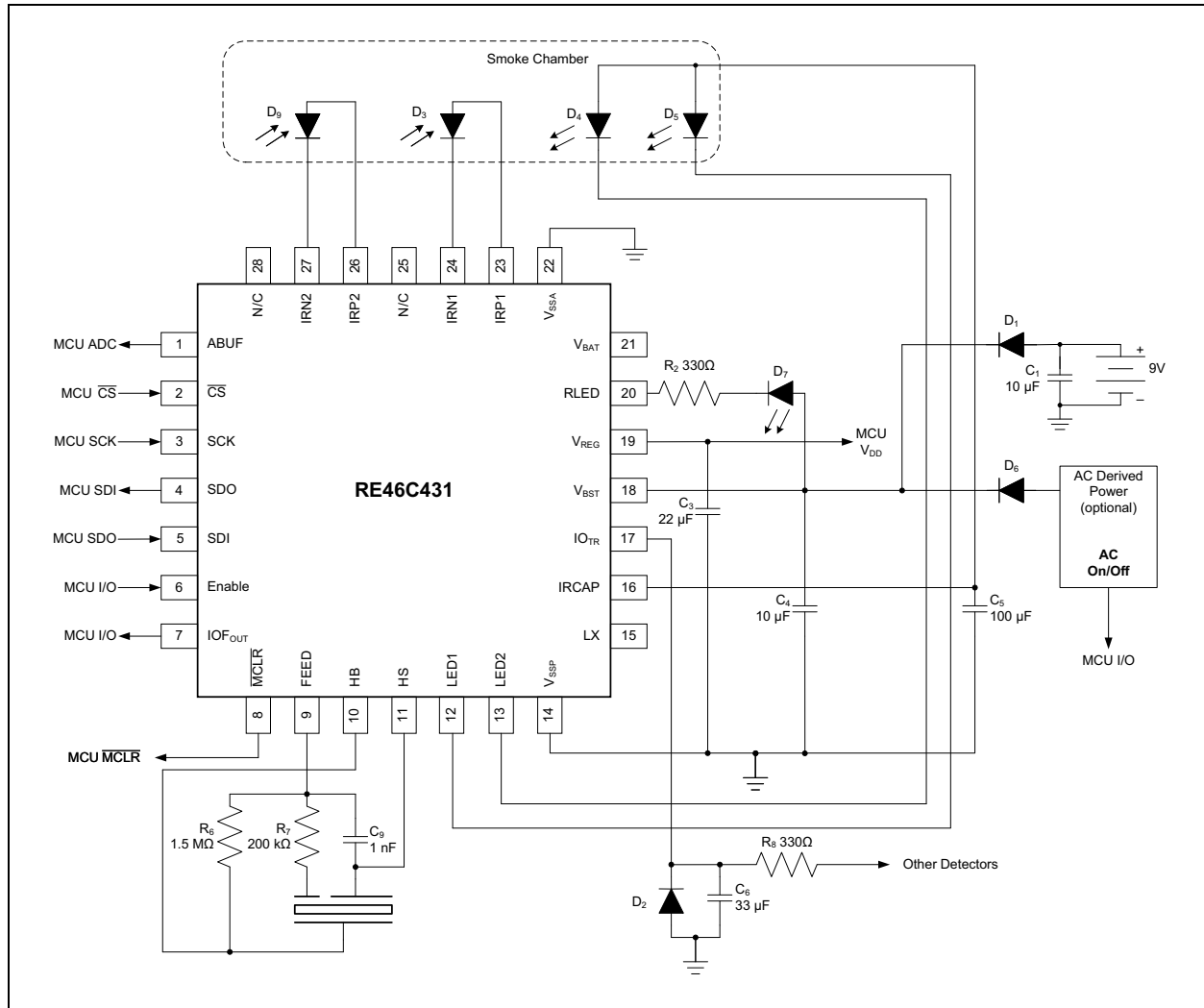
FIGURE 4-7: RE46C431 Typical 9V AC Application.
