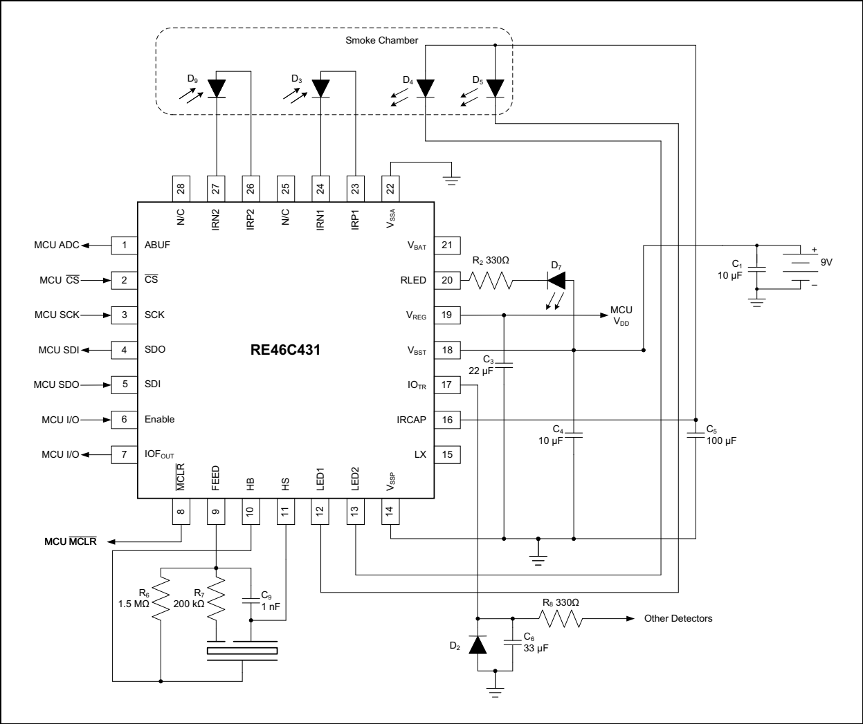
FIGURE 4-8: RE46C431 Typical 9V Application.
