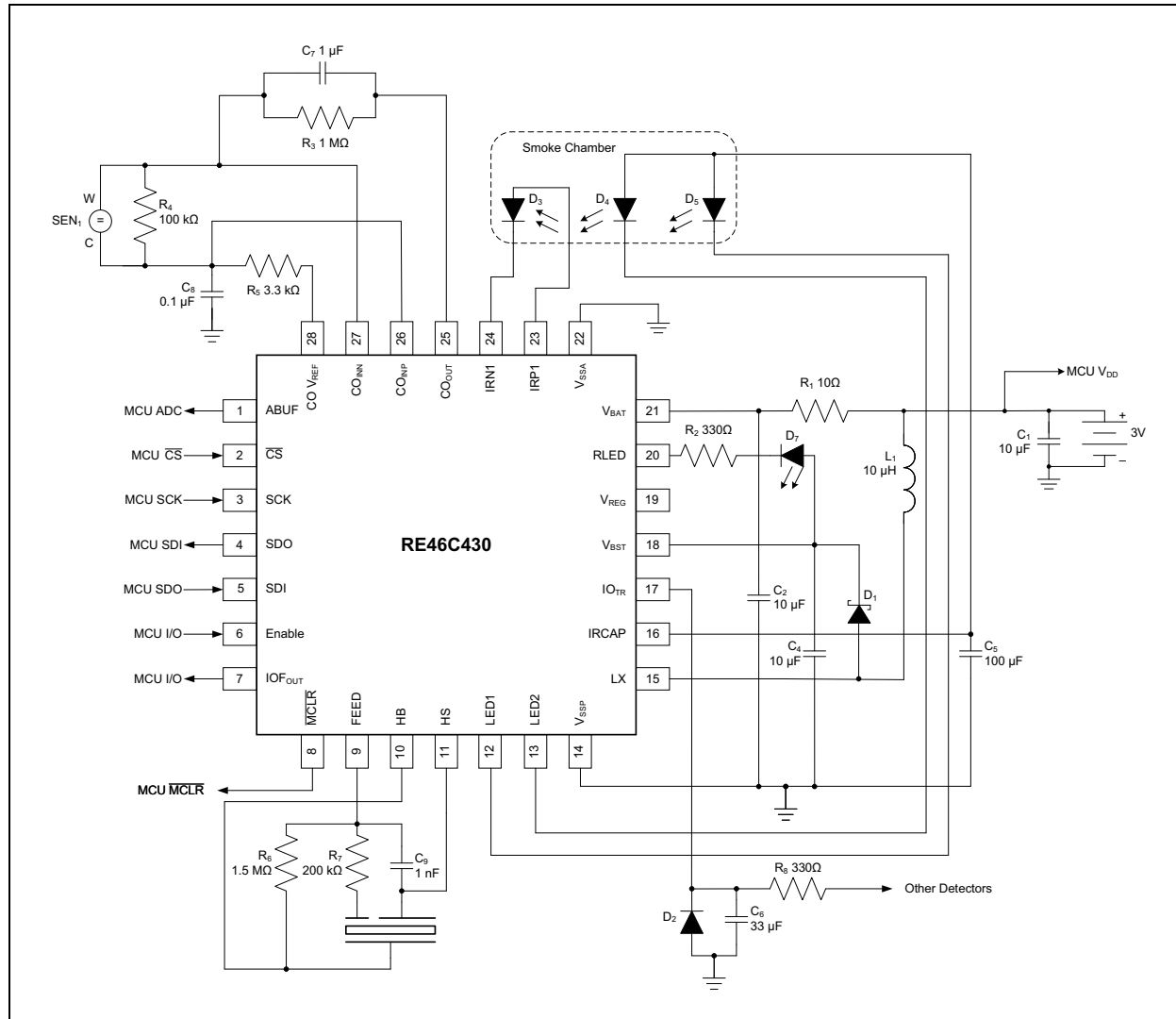
FIGURE 4-2: RE46C430 Typical 3V Battery-Only Application.
