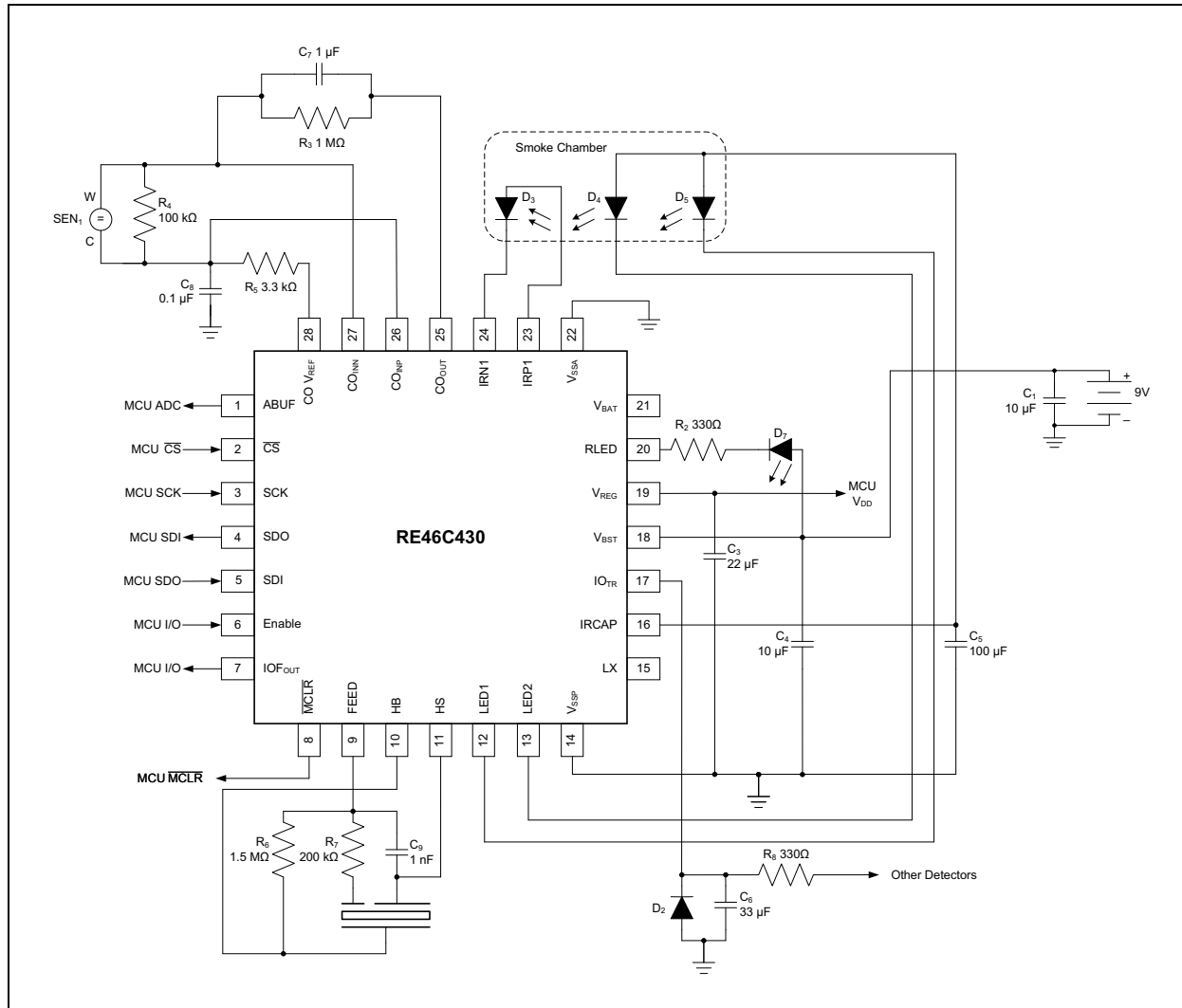
FIGURE 4-4: RE46C430 Typical 9V Battery-Only Application.
