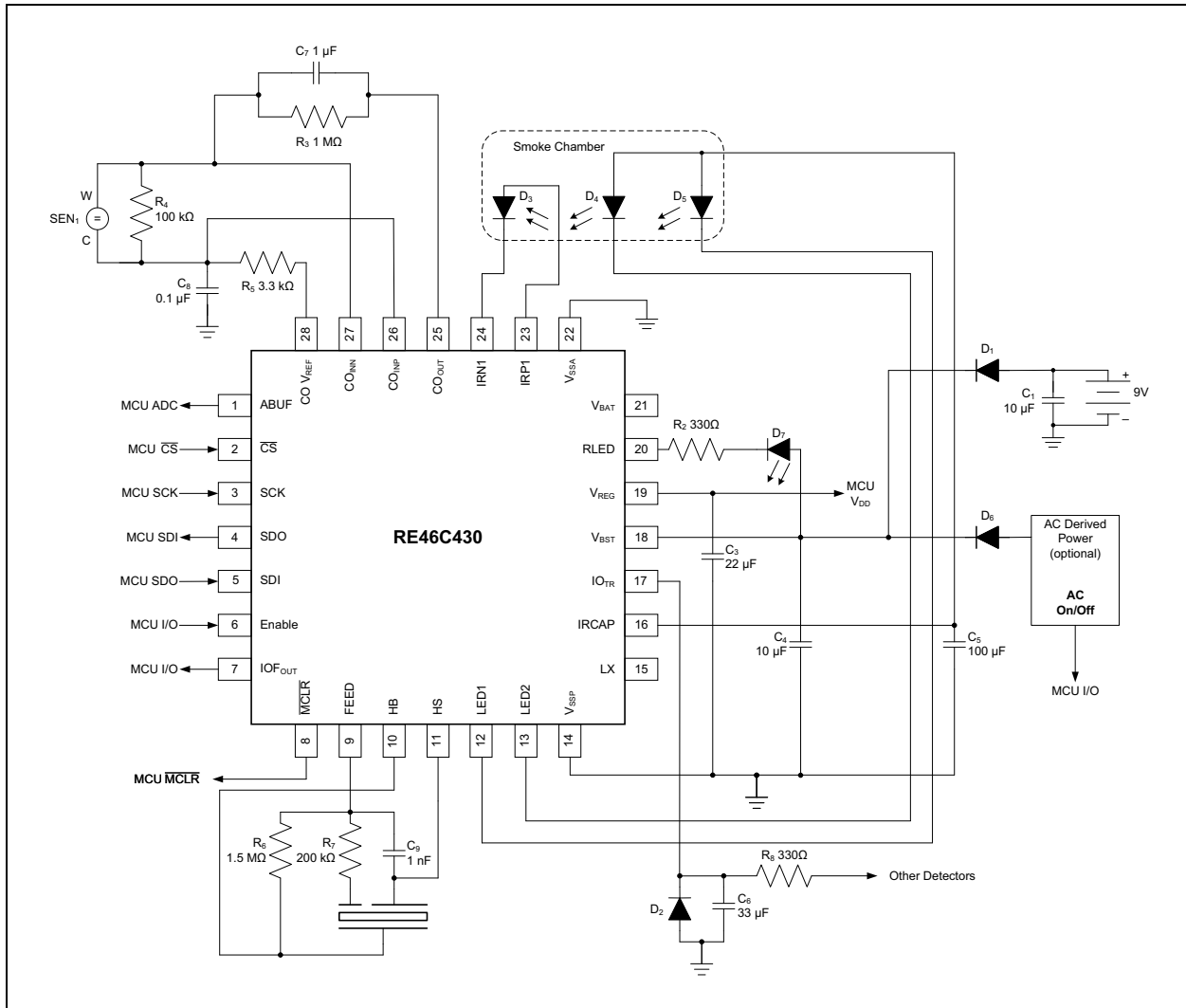
FIGURE 4-3: RE46C430 Typical 9V AC Application.
