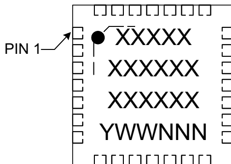
32-Lead VQFN, 5 x 5 x 1 mm (RE46C432)
