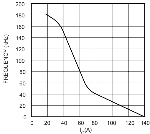
FIGURE 2, Max Frequency vs Current ( T_{\text{case}} = 75^{\circ}\text{C} )
