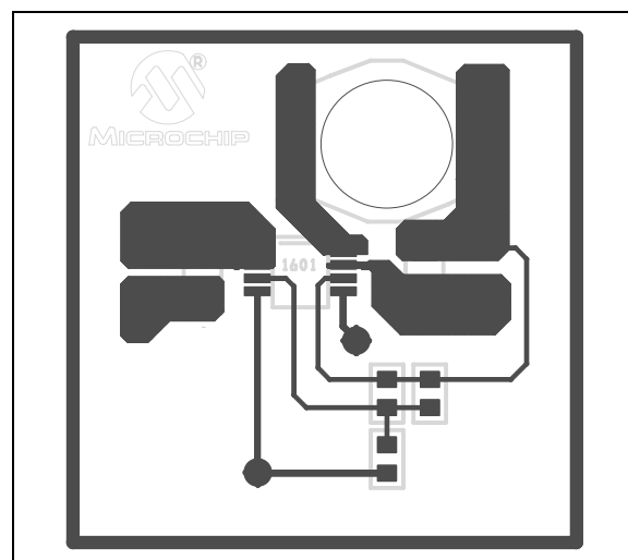
FIGURE 5-3: Top Layer.
