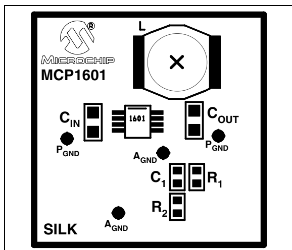
FIGURE 5-2: Component Placement.
