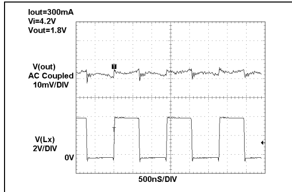
FIGURE 2-19: Typical Output Ripple Voltage (Forced PWM Mode).
