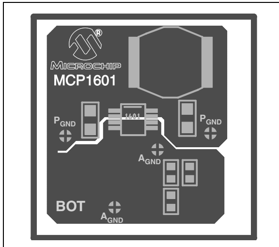
FIGURE 5-4: Bottom Layer.
