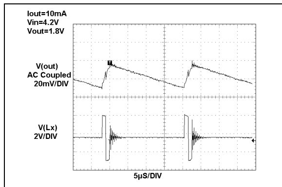
FIGURE 2-20: Typical Output Ripple Voltage (PFM Mode).
