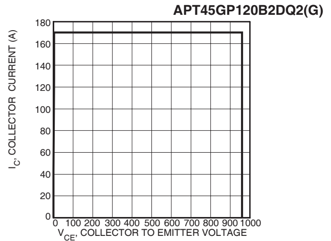
Figure 18, Minimum Reverse Bias Safe Operating Area
