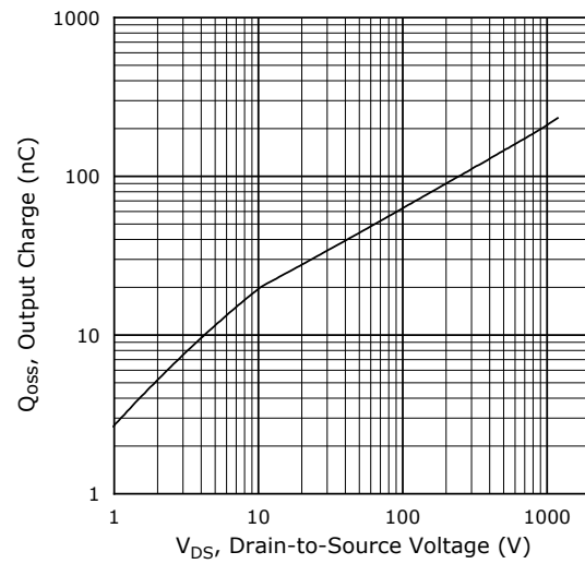
Figure 1-10. Q_{oss} vs. Drain-to-Source Voltage
