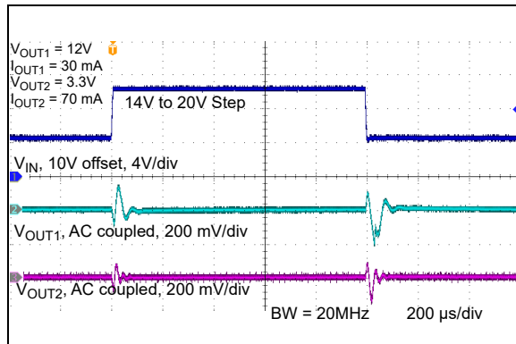
FIGURE 2-37: Dynamic Line Step ( V_R = 3.3\text{V} & V_R = 12\text{V} ).
