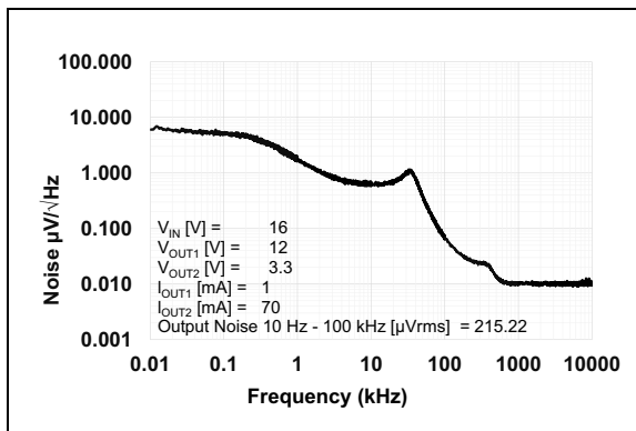
FIGURE 2-27: Noise vs. Frequency ( V_R = 3.3\text{V} ).
