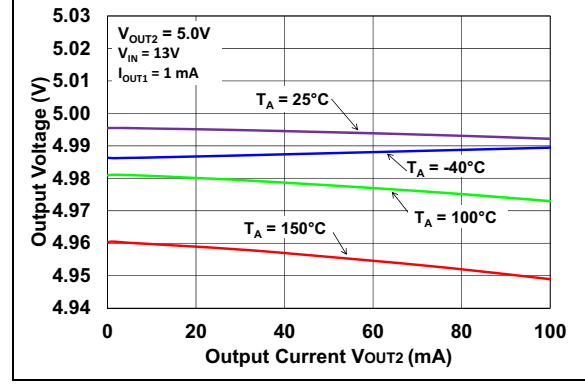
FIGURE 2-6: Output Voltage vs. Load Current ( V_R = 5.0\text{V} ).
