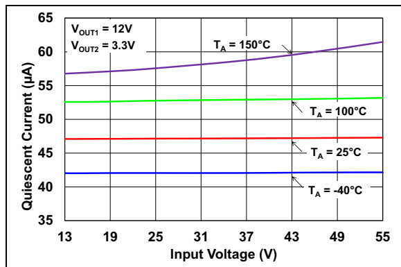
FIGURE 2-19: Quiescent Current vs. Input voltage ( V_R = 3.3\text{V} & V_R = 12\text{V} ).
