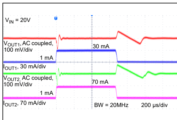
FIGURE 2-36: Dynamic Load Step ( V_R = 5.0\text{V} & V_R = 10\text{V} ).
