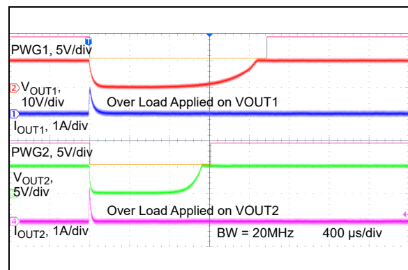
FIGURE 2-42: Power Good Fault Trigger ( V_R=5\text{V} & V_R=10\text{V} ).
