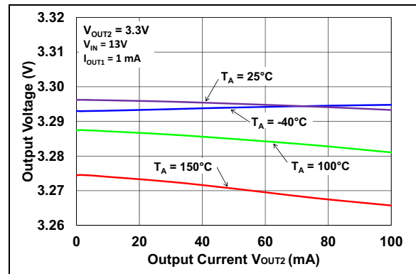
FIGURE 2-5: Output Voltage vs. Load Current ( V_R = 3.3\text{V} ).
