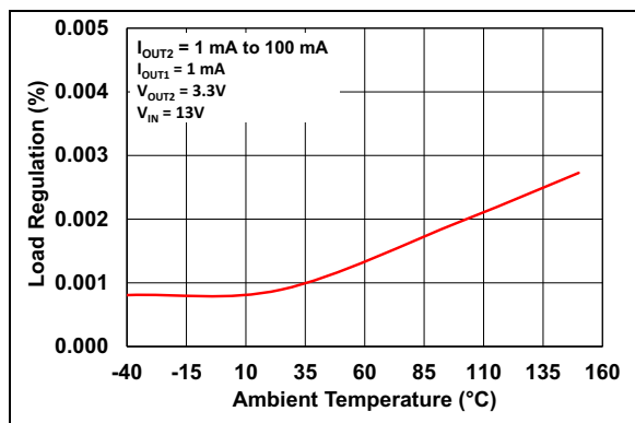
FIGURE 2-11: Load Regulation vs. Ambient Temperature ( V_R = 3.3\text{V} ).
