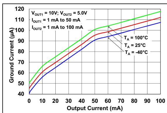
FIGURE 2-24: Ground Current vs. Load Current ( V_R = 5.0\text{V} & V_R = 10\text{V} ).
