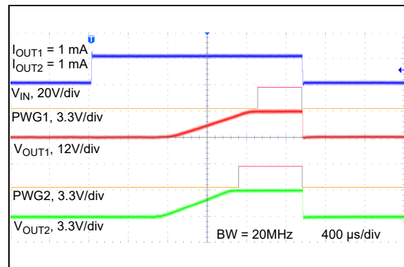
FIGURE 2-41: Power Good Transition ( V_R=3.3\text{V} & V_R=12\text{V} ).
