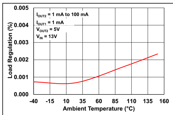
FIGURE 2-12: Load Regulation vs. Ambient Temperature ( V_R = 5.0\text{V} ).
