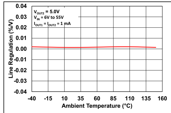
FIGURE 2-16: Line Regulation vs. Ambient Temperature ( V_R = 5.0\text{V} ).
