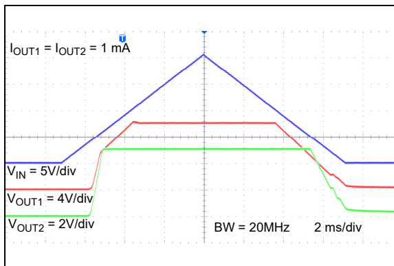
FIGURE 2-26: UVLO ( V_R = 5.0\text{V} & V_R = 10\text{V} ).
