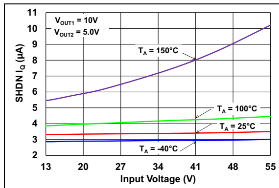
FIGURE 2-22: SHDN Quiescent Current vs. Input voltage ( V_R = 5.0\text{V} & V_R = 10\text{V} ).
