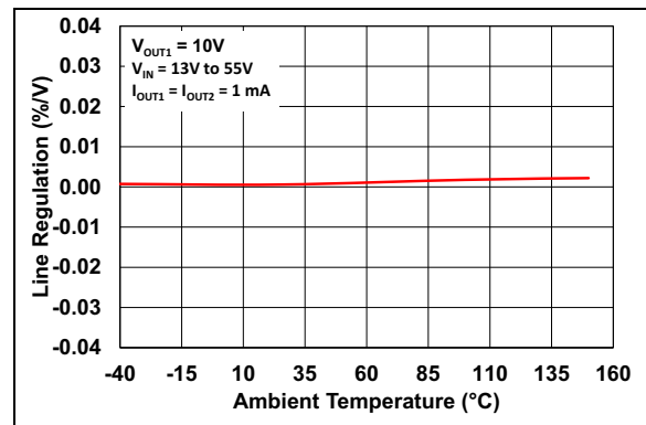
FIGURE 2-17: Line Regulation vs. Ambient Temperature ( V_R = 10\text{V} ).
