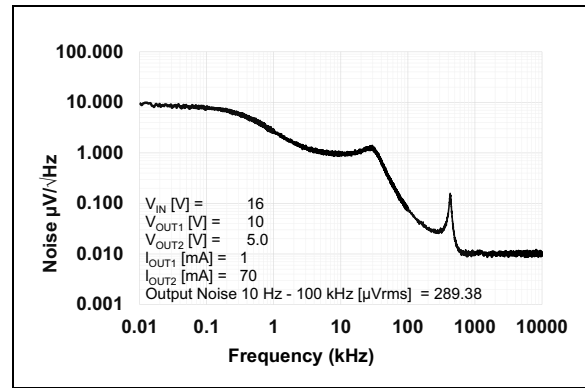
FIGURE 2-28: Noise vs. Frequency ( V_R = 5.0\text{V} ).
