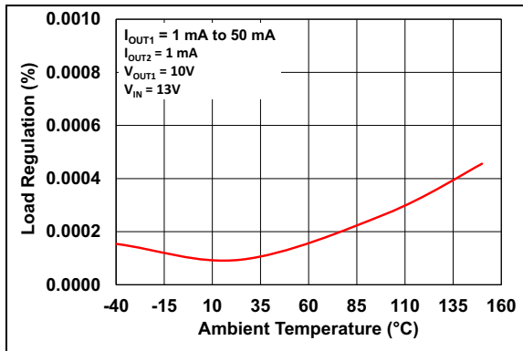
FIGURE 2-13: Load Regulation vs. Ambient Temperature ( V_R = 10\text{V} ).
