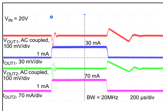
FIGURE 2-35: Dynamic Load Step ( V_R = 3.3\text{V} & V_R = 12\text{V} ).
