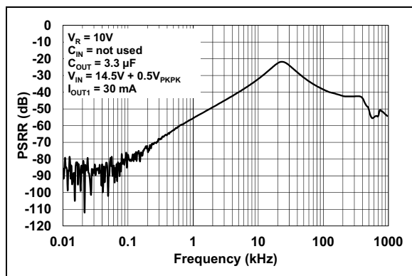
FIGURE 2-33: PSRR vs. Frequency ( V_R = 10\text{V} ).
