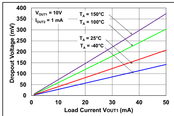
FIGURE 2-9: Dropout Voltage vs. Load Current ( V_R = 10\text{V} ).
