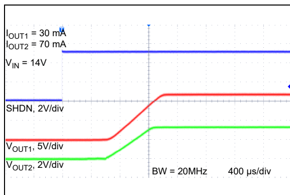
FIGURE 2-39: Start-up from SHDN (0V to 5V) ( V_R = 3.3\text{V} & V_R = 12\text{V} )
