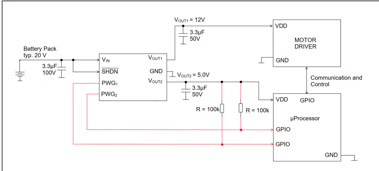
FIGURE 5-1: Typical Application Circuit II.
