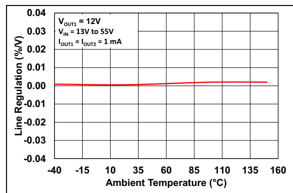
FIGURE 2-18: Line Regulation vs. Ambient Temperature ( V_R = 12\text{V} ).
