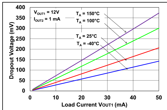
FIGURE 2-10: Dropout Voltage vs. Load Current ( V_R = 12\text{V} ).
