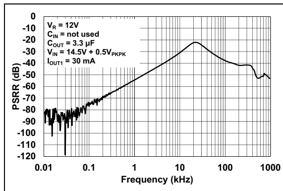
FIGURE 2-34: PSRR vs. Frequency ( V_R = 12\text{V} ).
