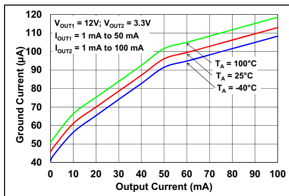
FIGURE 2-23: Ground Current vs. Load Current ( V_R = 3.3\text{V} & V_R = 12\text{V} ).
