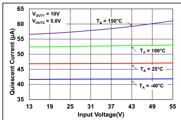
FIGURE 2-20: Quiescent Current vs. Input Voltage ( V_R = 5.0\text{V} & V_R = 10\text{V} ).
