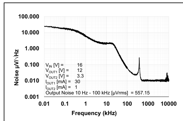
FIGURE 2-30: Noise vs. Frequency ( V_R = 12\text{V} ).
