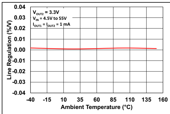
FIGURE 2-15: Line Regulation vs. Ambient Temperature ( V_R = 3.3\text{V} ).
