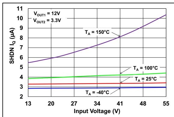
FIGURE 2-21: SHDN Quiescent Current vs. Input voltage ( V_R = 3.3\text{V} & V_R = 12\text{V} ).
