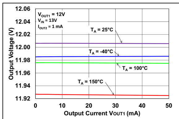
FIGURE 2-8: Output Voltage vs. Load Current ( V_R = 12\text{V} ).
