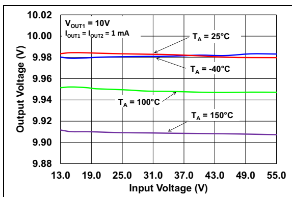
FIGURE 2-3: Output Voltage vs Input Voltage ( V_R = 10\text{V} ).
