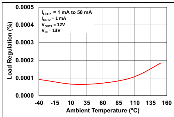
FIGURE 2-14: Load Regulation vs. Ambient Temperature ( V_R = 12\text{V} ).
