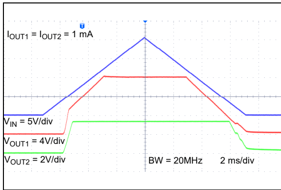
FIGURE 2-25: UVLO ( V_R = 3.3\text{V} & V_R = 12\text{V} ).
