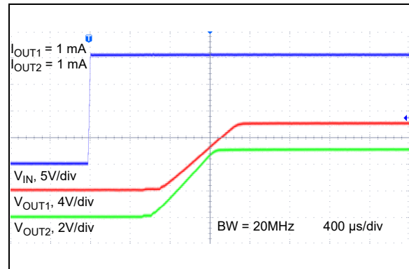
FIGURE 2-40: Start-up from V_{IN} (0V to 14V) ( V_R = 5\text{V} & V_R = 10\text{V} )
