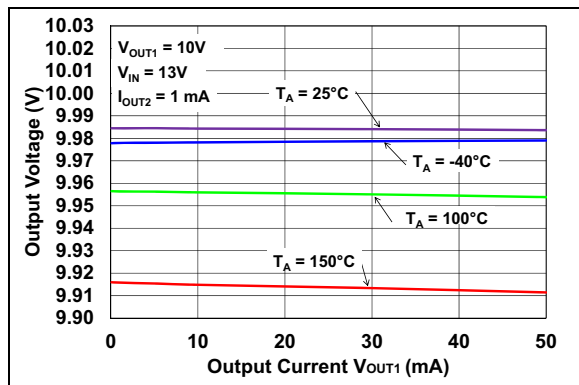
FIGURE 2-7: Output Voltage vs. Load Current ( V_R = 10\text{V} ).
