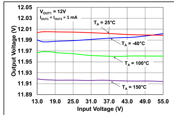
FIGURE 2-4: Output Voltage vs Input voltage ( V_R = 12\text{V} ).
