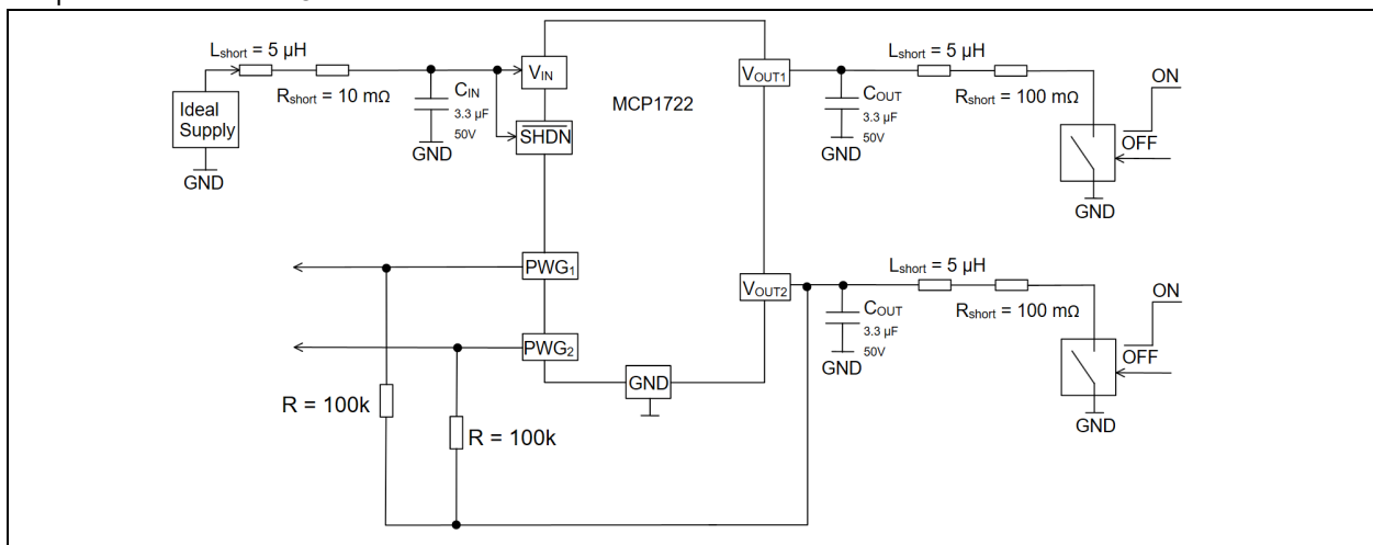
FIGURE 4-2: Short Circuit Test Set-Up.
