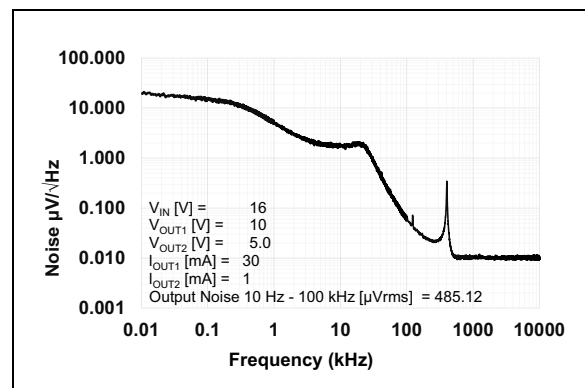
FIGURE 2-29: Noise vs. Frequency ( V_R = 10\text{V} ).
