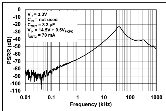
FIGURE 2-31: PSRR vs. Frequency ( V_R = 3.3\text{V} ).
