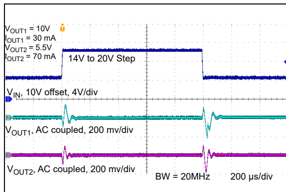
FIGURE 2-38: Dynamic Line Step ( V_R = 3.3\text{V} & V_R = 12\text{V} ).
