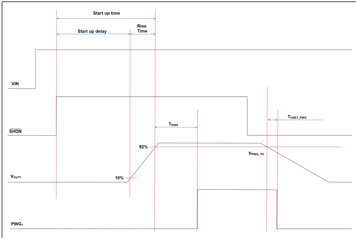
FIGURE 4-3: Timing Diagram.
