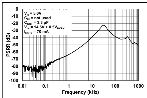
FIGURE 2-32: PSRR vs. Frequency ( V_R = 5.0\text{V} ).
