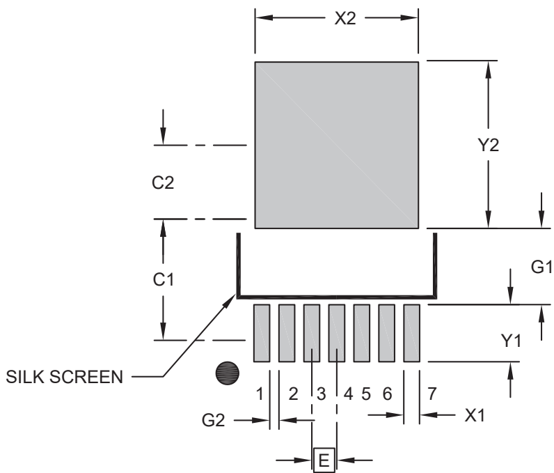
Figure 2-2. Recommended Land Pattern
