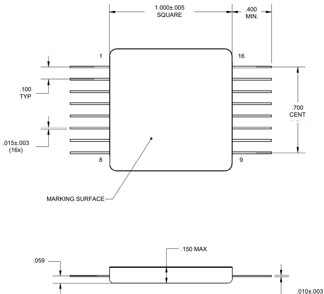
Figure 6-4. Model 1319 Package Outline and I/O Connection
