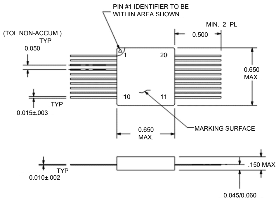
Figure 6-2. Model 1304/1308 Package Outline and I/O Connection
