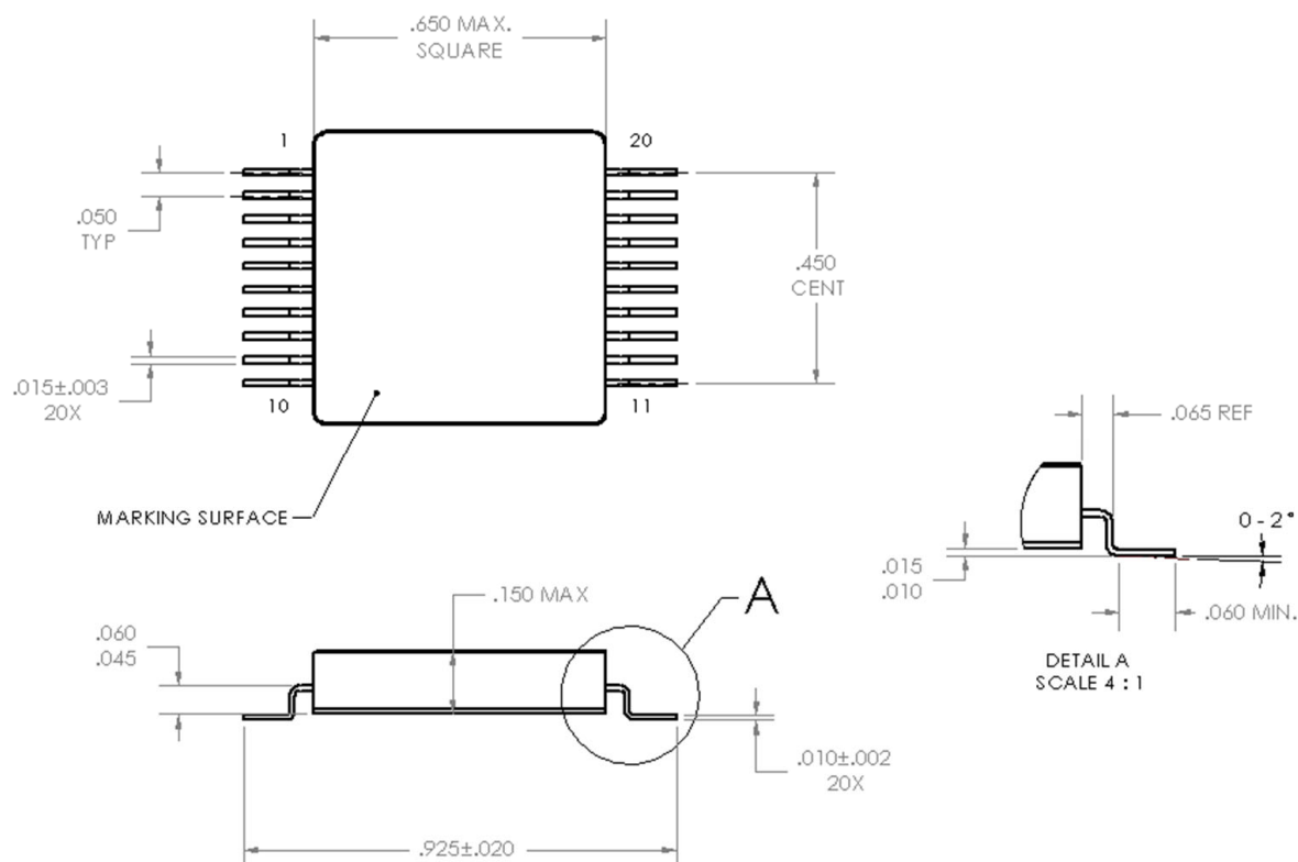
Figure 6-3. Model 1320/1340 Package Outline and I/O Connection
