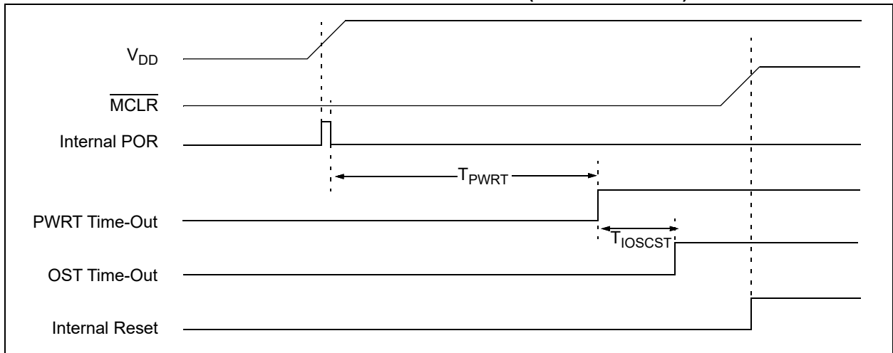
FIGURE 13-6: TIME-OUT SEQUENCE ON POWER-UP (MCLR WITH V DD )
