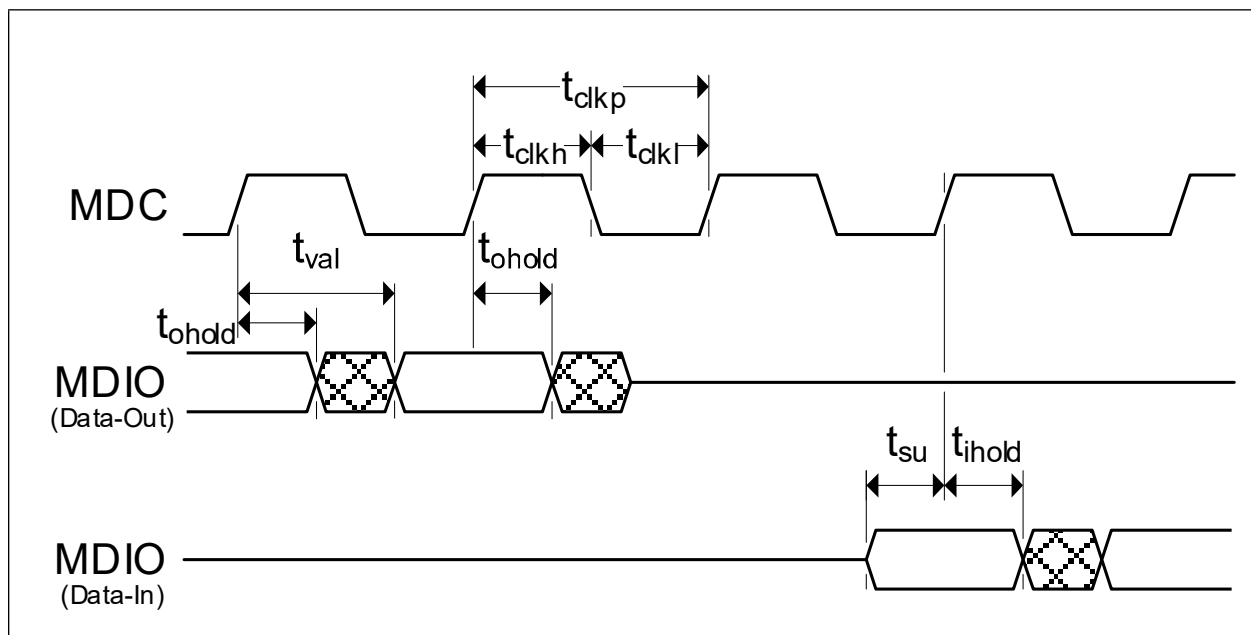
FIGURE 4-2: MDC/MDIO TIMING
