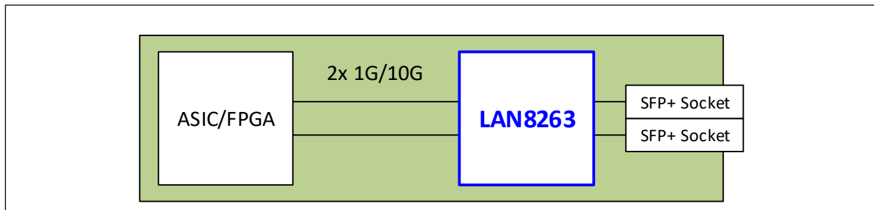
FIGURE 1-2: PHY WITH HIGH-ACCURACY 1588 TIMESTAMPING
