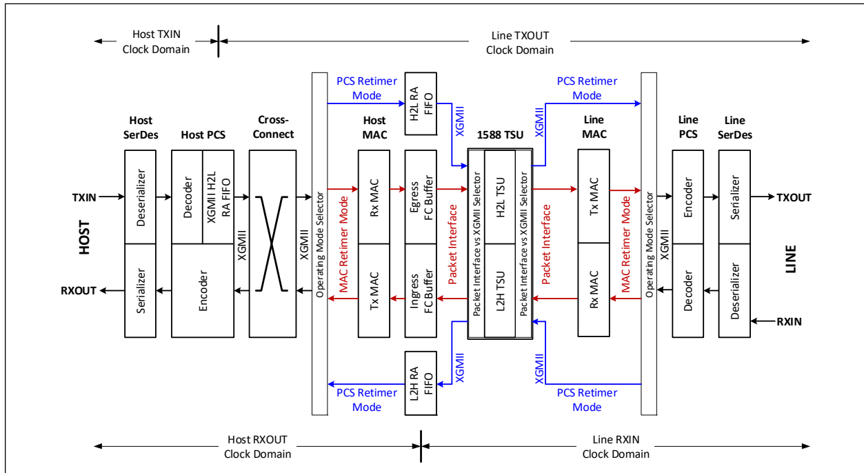
FIGURE 3-1: LAN8263 DATA PATH
