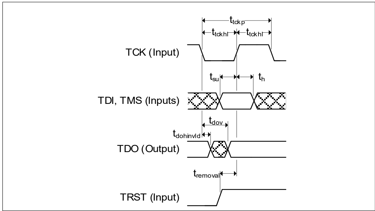
FIGURE 4-12: JTAG TIMING
