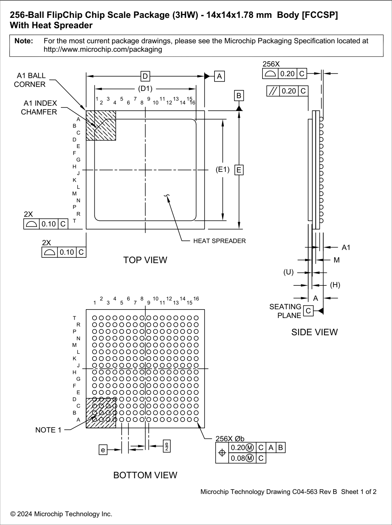
FIGURE 5-1: 256-BGA PACKAGE DRAWING
