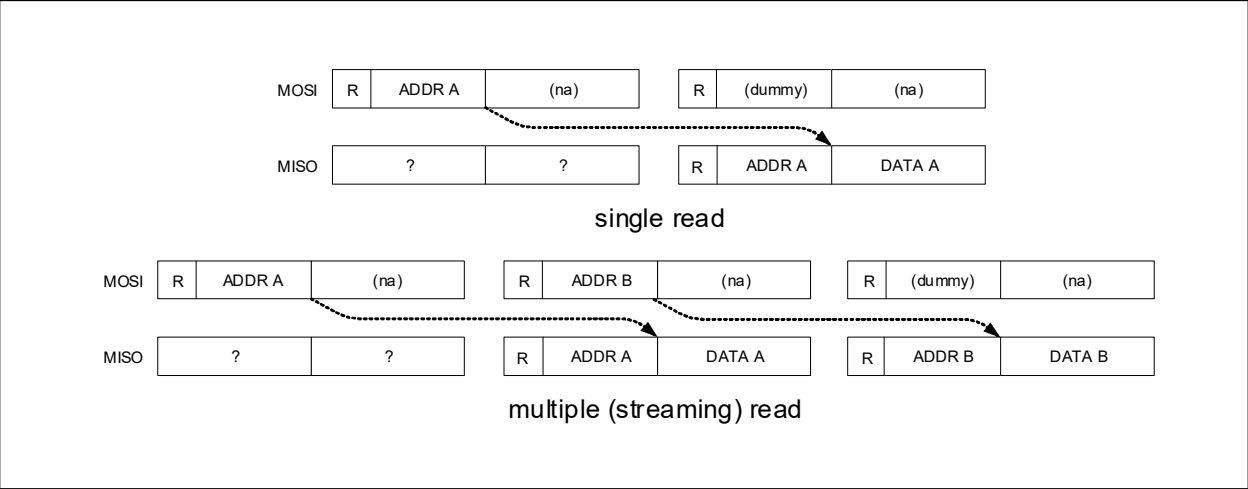
FIGURE 3-30: SPI CLIENT PIPELINED READS
