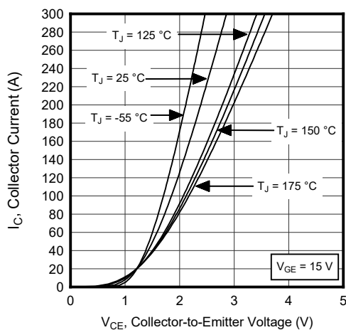
Figure 1-1. Output Characteristics
