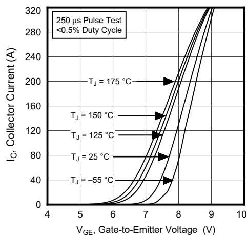
Figure 1-2. Transfer Characteristics
