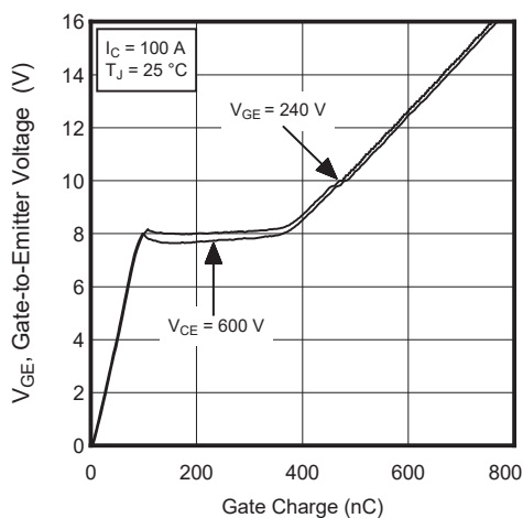
Figure 1-3. Gate Charge
