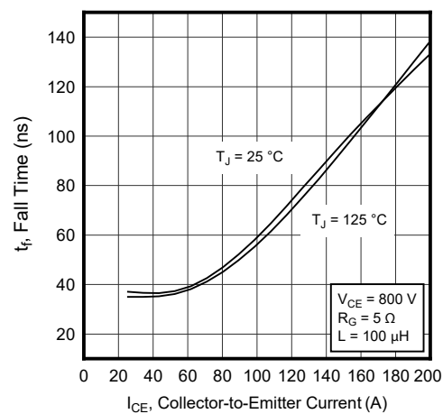
Figure 1-10. Current Fall Time vs. Collector Current
