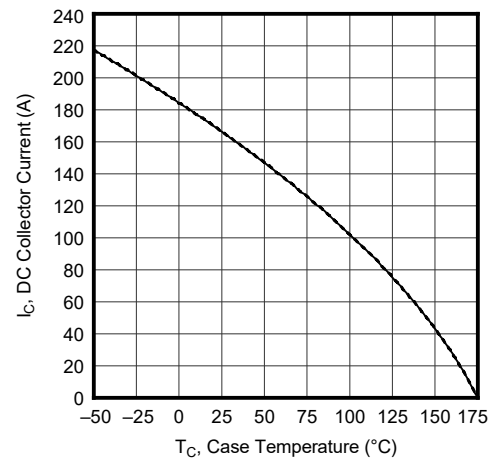
Figure 1-6. DC Collector Current vs. Case Temperature
