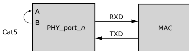
FIGURE 5-19: CONNECTOR LOOPBACK DIAGRAM
