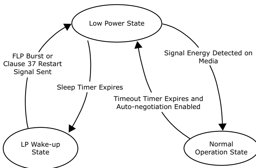
FIGURE 5-11: ACTIPHY STATE DIAGRAM
