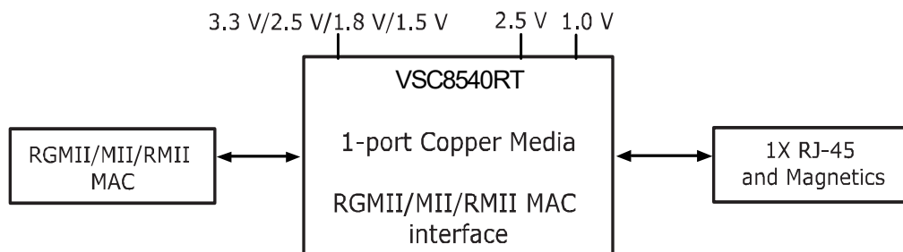
FIGURE 1: APPLICATION DIAGRAM
