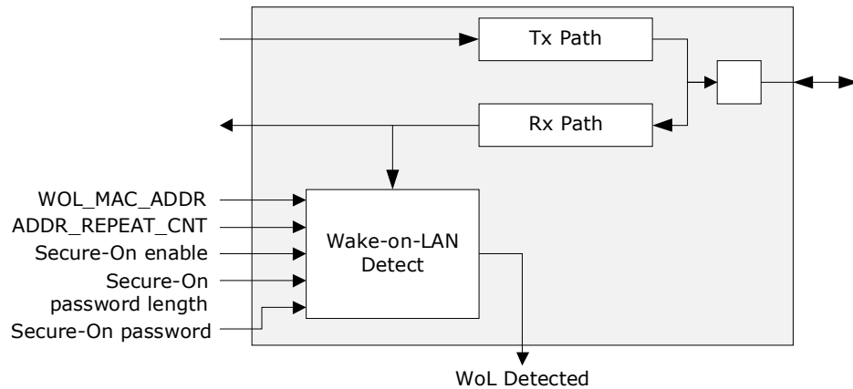
FIGURE 5-15: WAKE-ON-LAN FUNCTIONALITY
