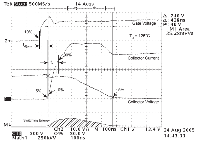
Figure 22, Turn-on Switching Waveforms and Definitions
