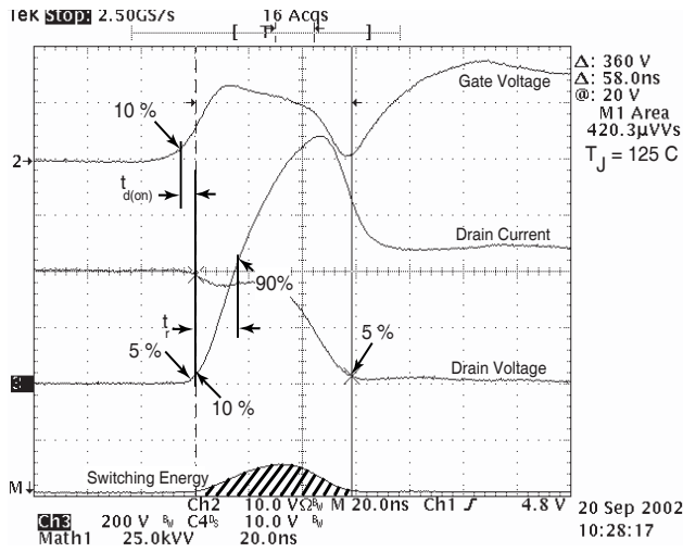
Figure 18, Turn-on Switching Waveforms and Definitions
