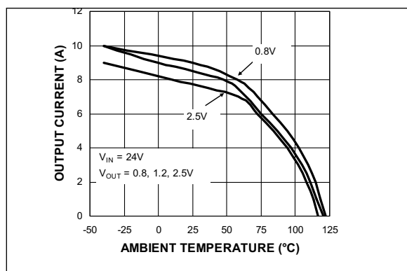
FIGURE 2-39: Thermal Derating* vs. Ambient Temperature.
