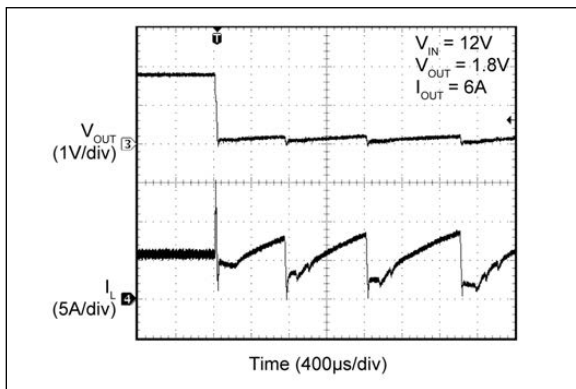
FIGURE 2-50: Short Circuit.
