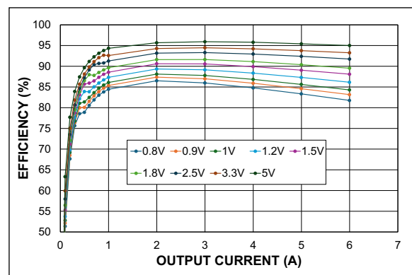
FIGURE 2-29: Efficiency ( V_{IN} = 12V ) vs. Output Current.
