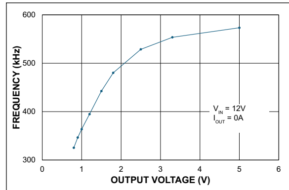
FIGURE 2-24: Switching Frequency vs. Output Voltage.
