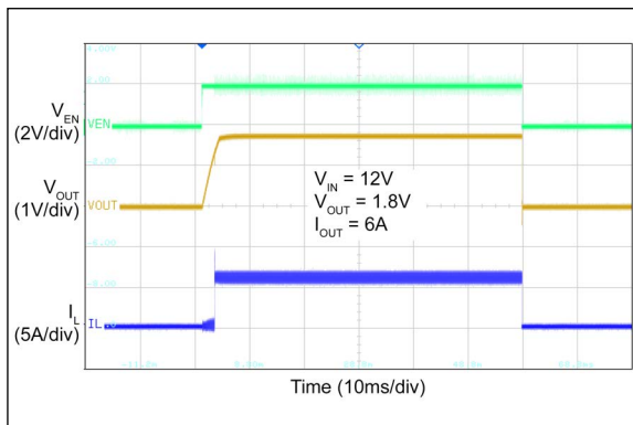
FIGURE 2-45: Enable Turn-On/Turn-Off.
