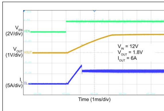
FIGURE 2-42: Enable Turn-On Delay and Rise Time.
