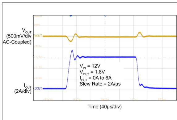
FIGURE 2-56: Transient Response.
