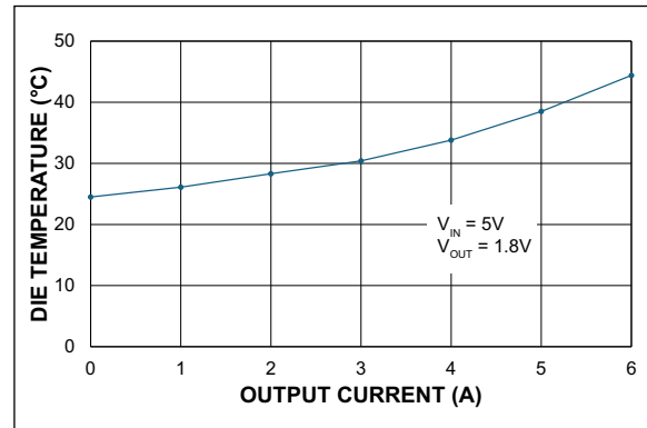
FIGURE 2-28: Die Temperature* ( V_{IN} = 5V ) vs. Output Current.
