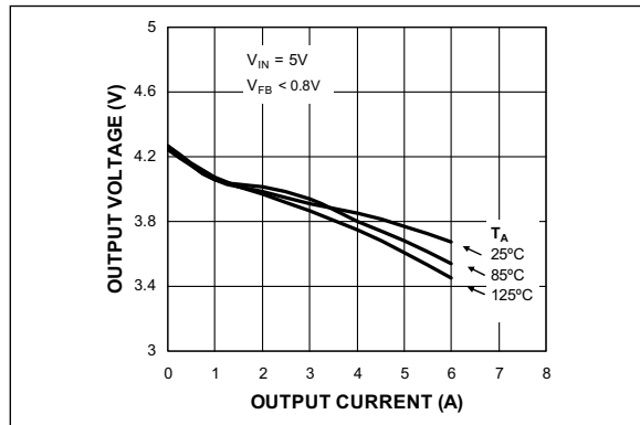
FIGURE 2-25: Output Voltage ( V_{IN} = 5V ) vs. Output Current.
