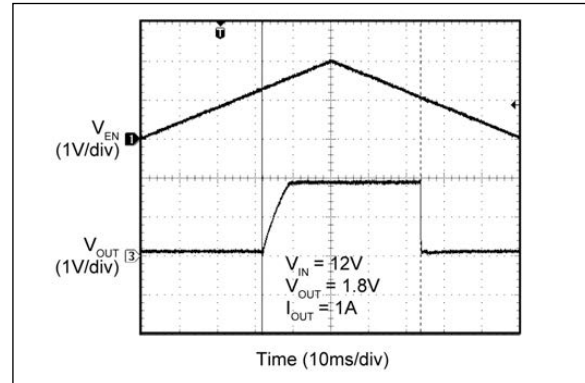
FIGURE 2-46: Enable Thresholds.
