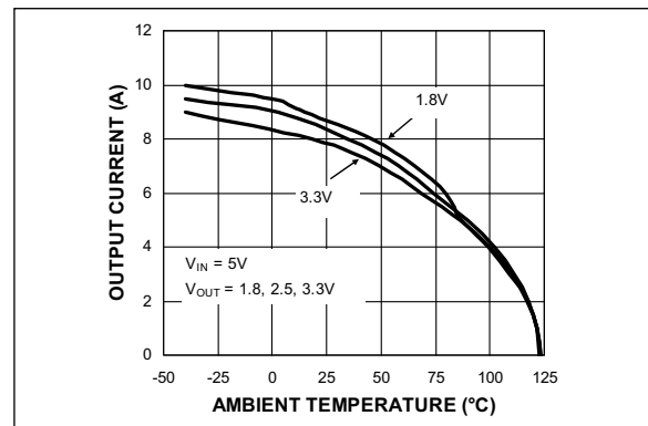
FIGURE 2-36: Thermal Derating* vs. Ambient Temperature.
