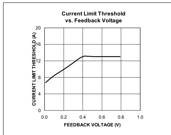
FIGURE 4-3: Current Limit Foldback Characteristic.
