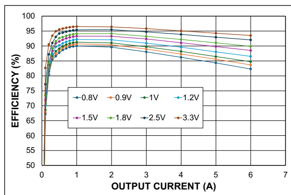
FIGURE 2-26: Efficiency ( V_{IN} = 5V ) vs. Output Current.
