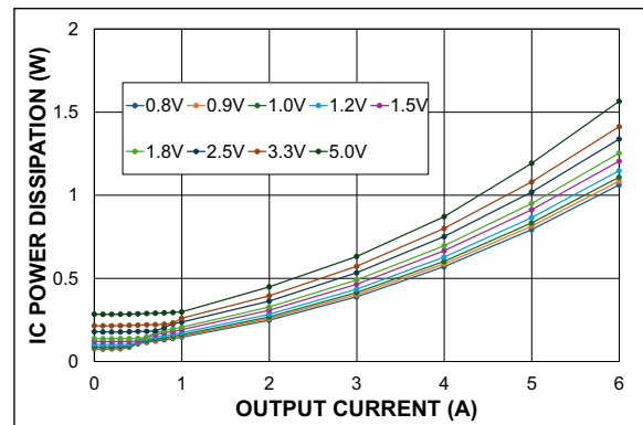
FIGURE 2-30: IC Power Dissipation ( V_{IN} = 12V ) vs. Output Current.
