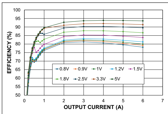
FIGURE 2-32: Efficiency ( V_{IN} = 24V ) vs. Output Current.
