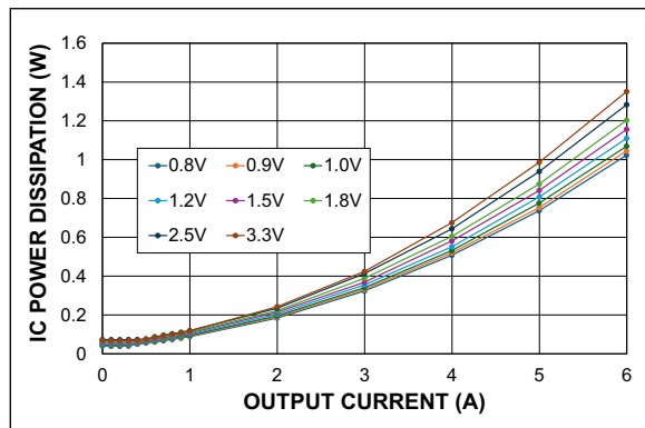
FIGURE 2-27: IC Power Dissipation ( V_{IN} = 5V ) vs. Output Current.
