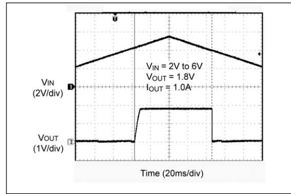
FIGURE 2-47: V_IN UVLO Thresholds.
