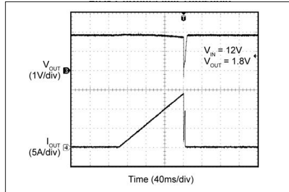
FIGURE 2-52: Peak Current Limit Threshold.
