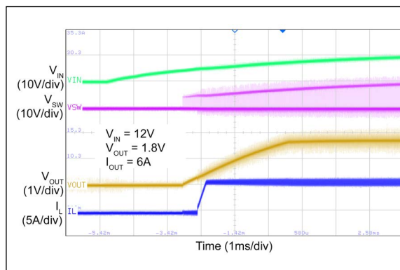
FIGURE 2-40: V_{IN} Soft Turn-On.
