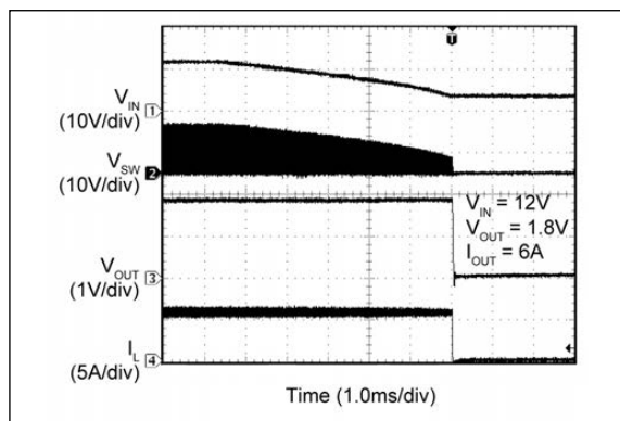
FIGURE 2-41: V_{IN} Soft Turn-Off.
