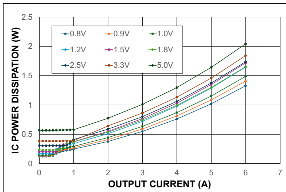
FIGURE 2-33: IC Power Dissipation ( V_{IN} = 24V ) vs. Output Current.
