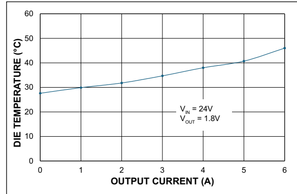
FIGURE 2-34: Die Temperature* ( V_{IN} = 24V ) vs. Output Current.
