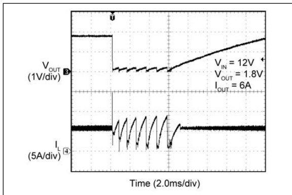
FIGURE 2-51: Output Recovery from Short Circuit.
