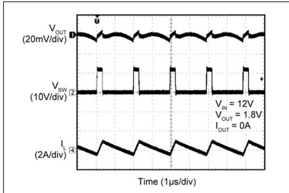
FIGURE 2-55: Switching Waveforms; I_{OUT} = 0A .
