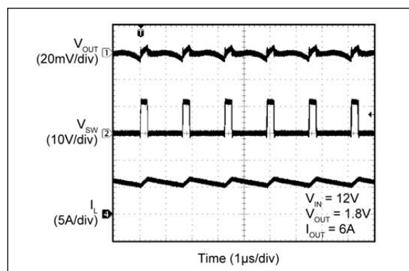
FIGURE 2-54: Switching Waveforms; I_{OUT} = 6A .
