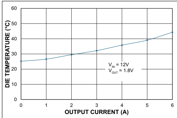
FIGURE 2-31: Die Temperature* ( V_{IN} = 12V ) vs. Output Current.
