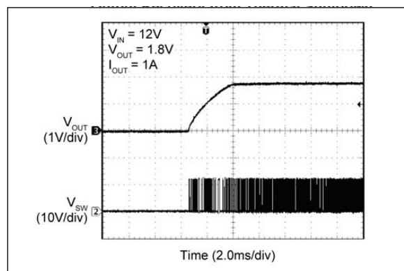
FIGURE 2-53: Output Recovery from Thermal Shutdown.
