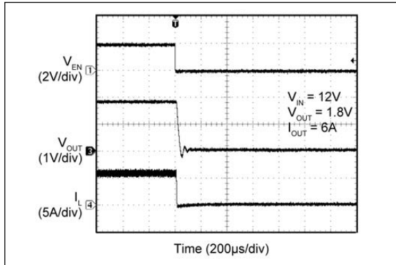
FIGURE 2-43: Enable Turn-Off Delay and Fall Time.
