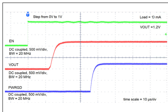
FIGURE 2-21: Enable Turn-On Time.
