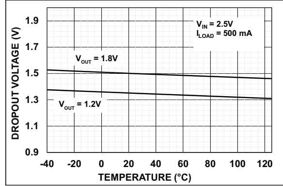
FIGURE 2-6: Bias Dropout Voltage vs. Temperature.
