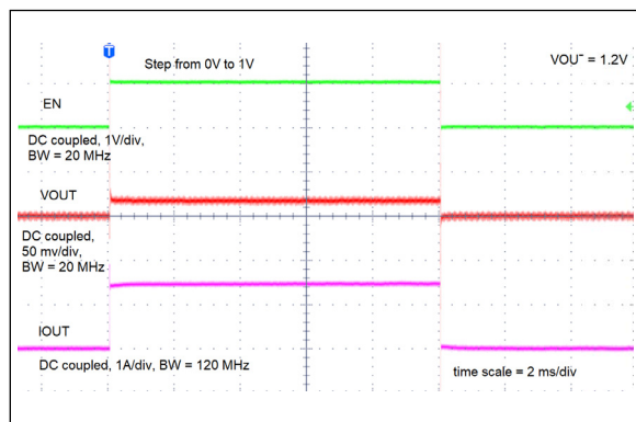
FIGURE 2-19: Enabled into Short-Circuit.
