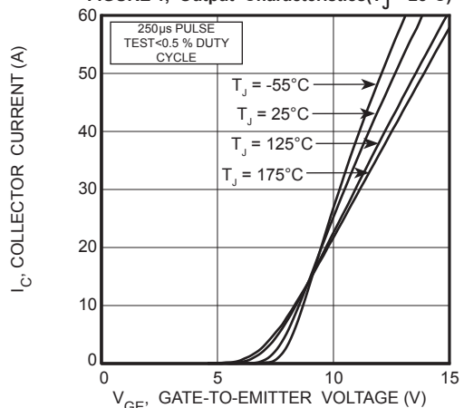
FIGURE 3, Transfer Characteristics
