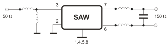
Topology 1 (default):
