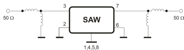
Topology 2:
