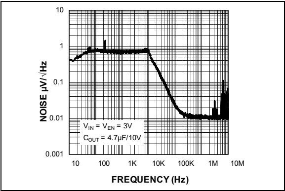
FIGURE 2-15: MIC94355YMT Output Noise Spectral Density.
