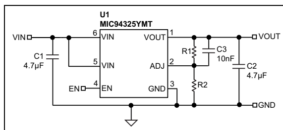
FIGURE 4-1: Adjustable Output Voltage.
