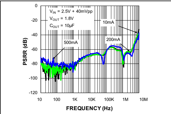
FIGURE 2-8: MIC94355 PSRR, C_{OUT} = 10\mu F .
