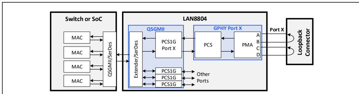
FIGURE 5-5: EXTERNAL CONNECTOR LOOPBACK
