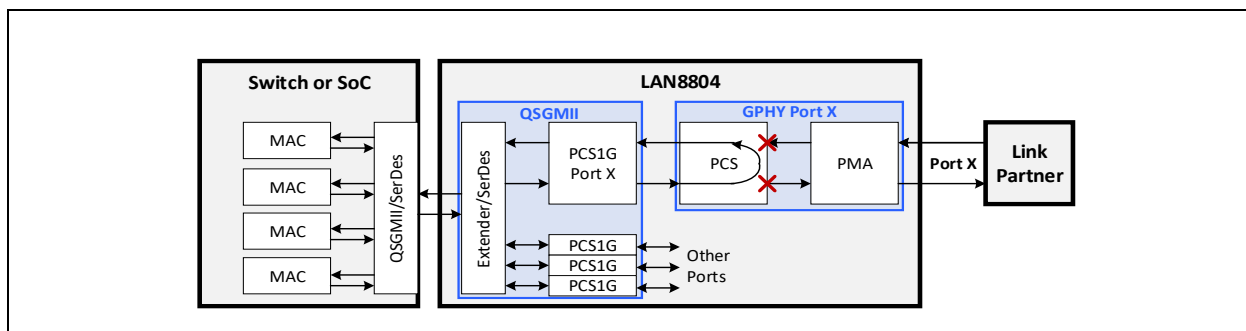
FIGURE 5-3: DIGITAL (NEAR-END) LOOPBACK
