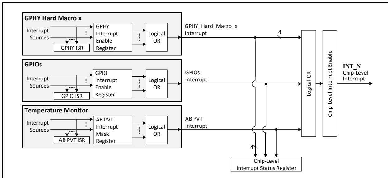
FIGURE 5-8: INTERRUPT STRUCTURE
