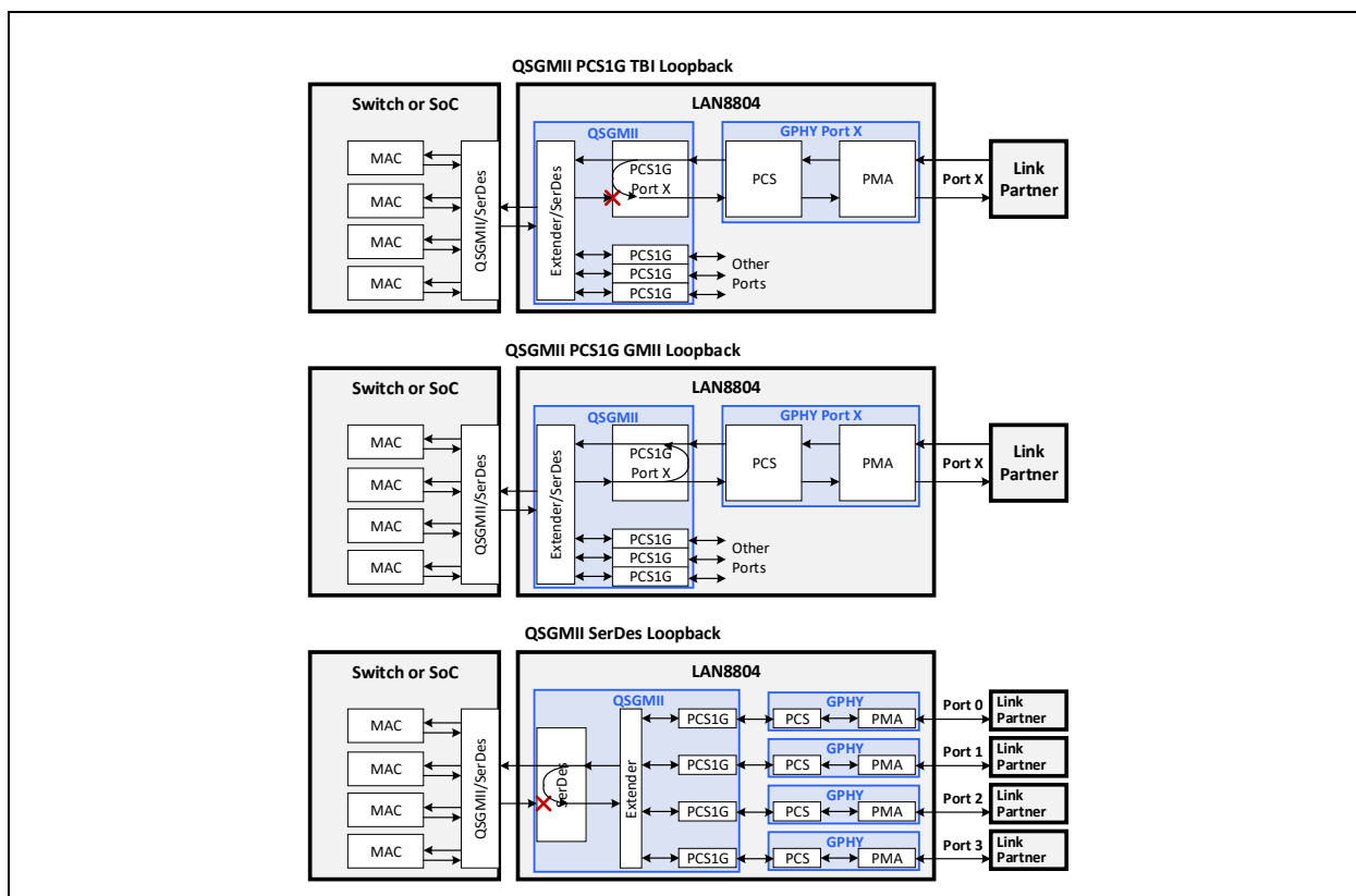
FIGURE 5-6: QSGMII LOOPBACK
