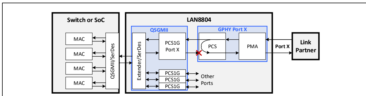
FIGURE 5-4: REMOTE (FAR-END) LOOPBACK
