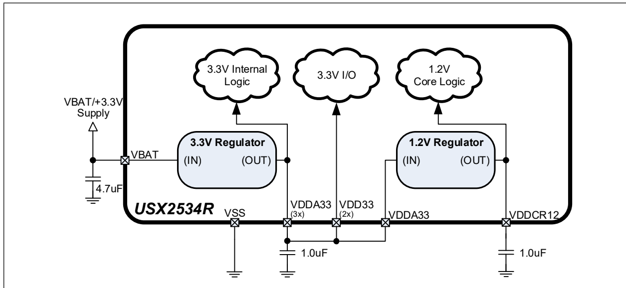
FIGURE 4-1: POWER CONNECTIONS
